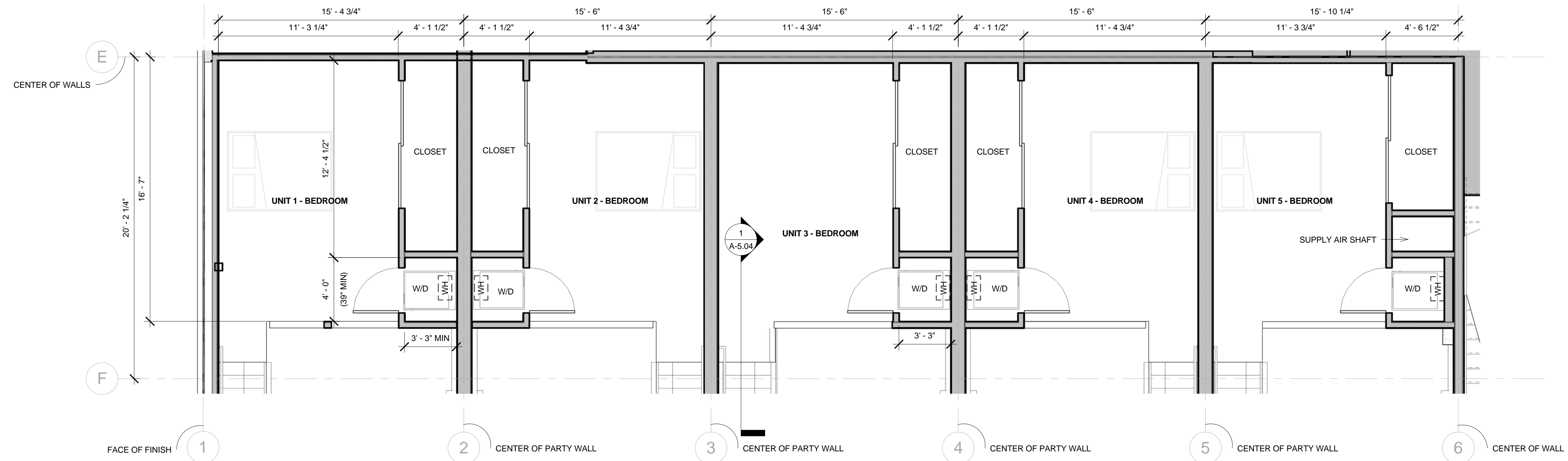
2 63RD STREET LOFTS - DECK SCALE: 1/4" = 1'-0"
