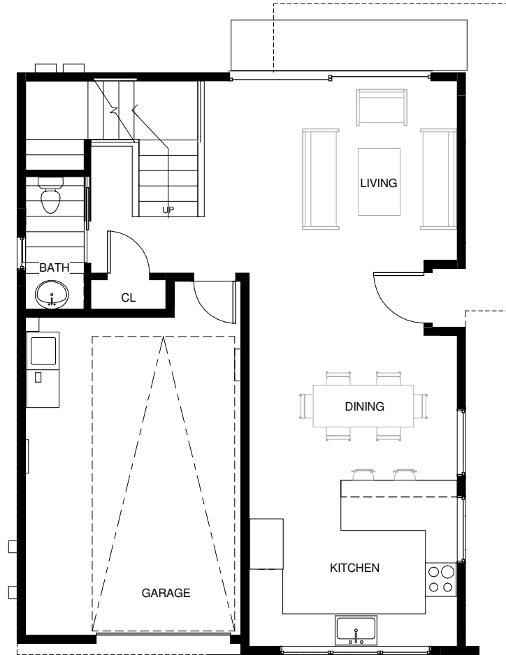
① 1696 16TH ST - LEVEL 1 1/4" = 1'-0"
