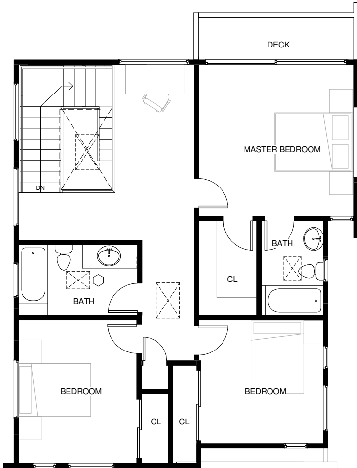
② 1696 16TH ST - LEVEL 2 1/4" = 1'-0"
