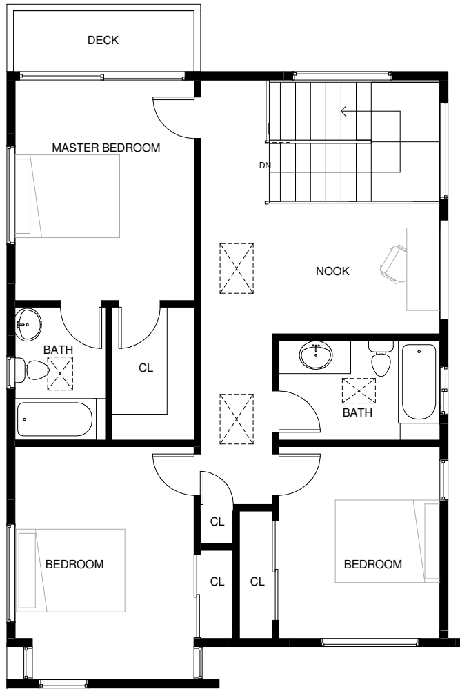
② 1606 WILLOW ST - LEVEL 2 1/4" = 1'-0"
