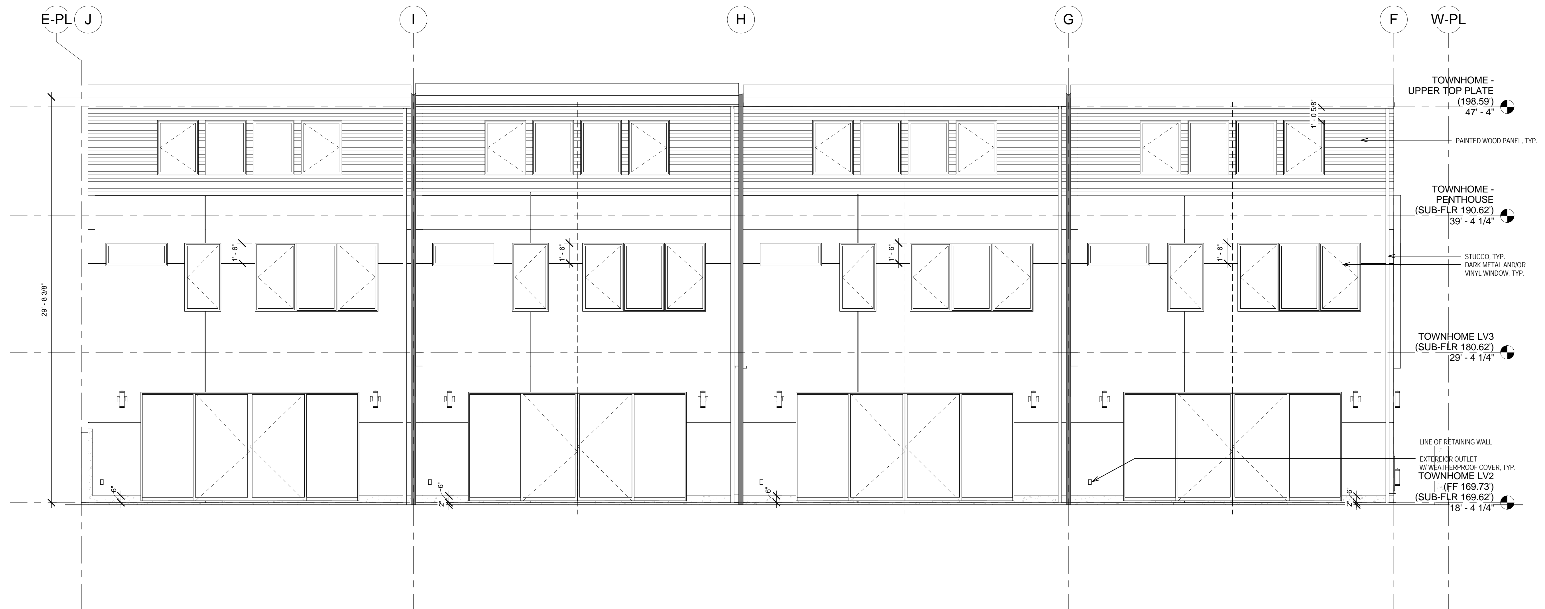
1 TOWNHOME NORTH ELEVATION SCALE: 1/4" = 1'-0"
