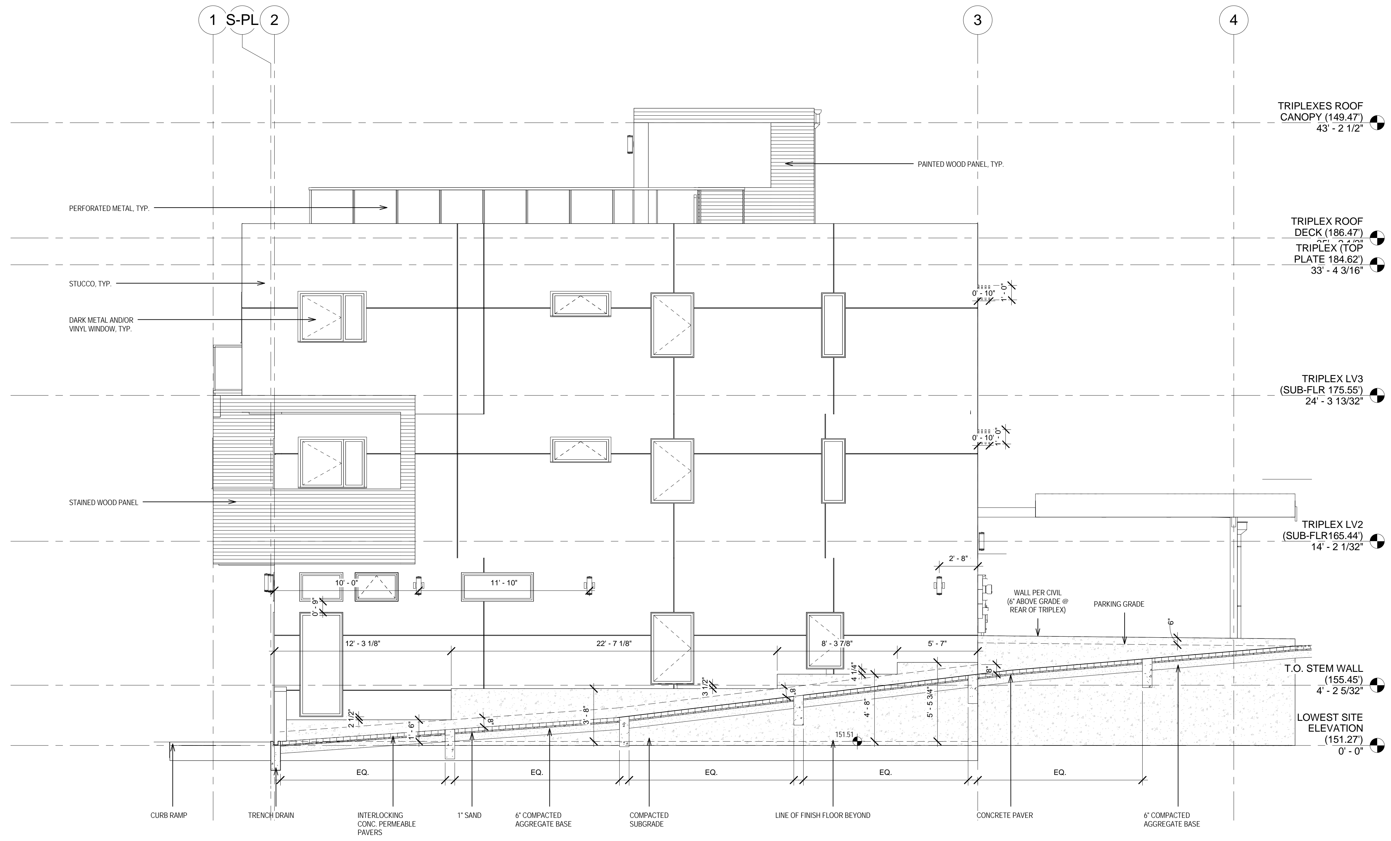
1 LOT 1 - EAST ELEVATION SCALE: 1/4" = 1'-0"
