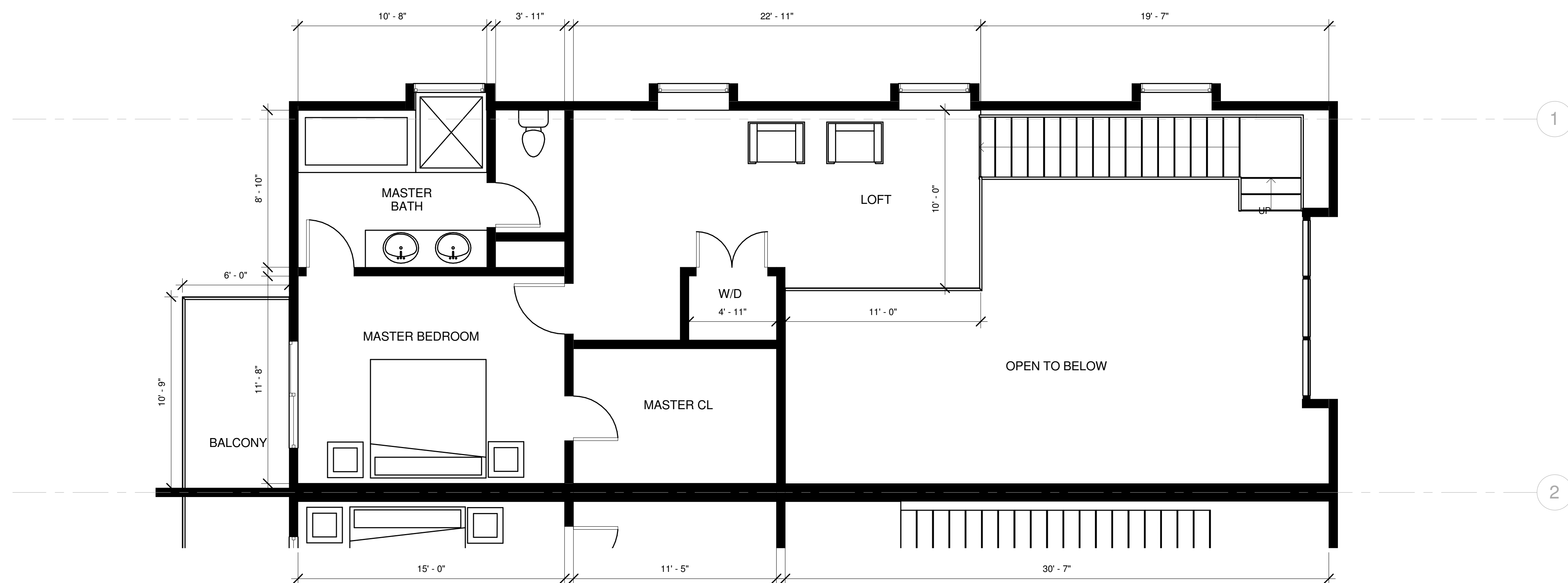
2 UNIT G1 ENLARGED PLAN LEVEL 2 SCALE: 1/4" = 1'-0"
