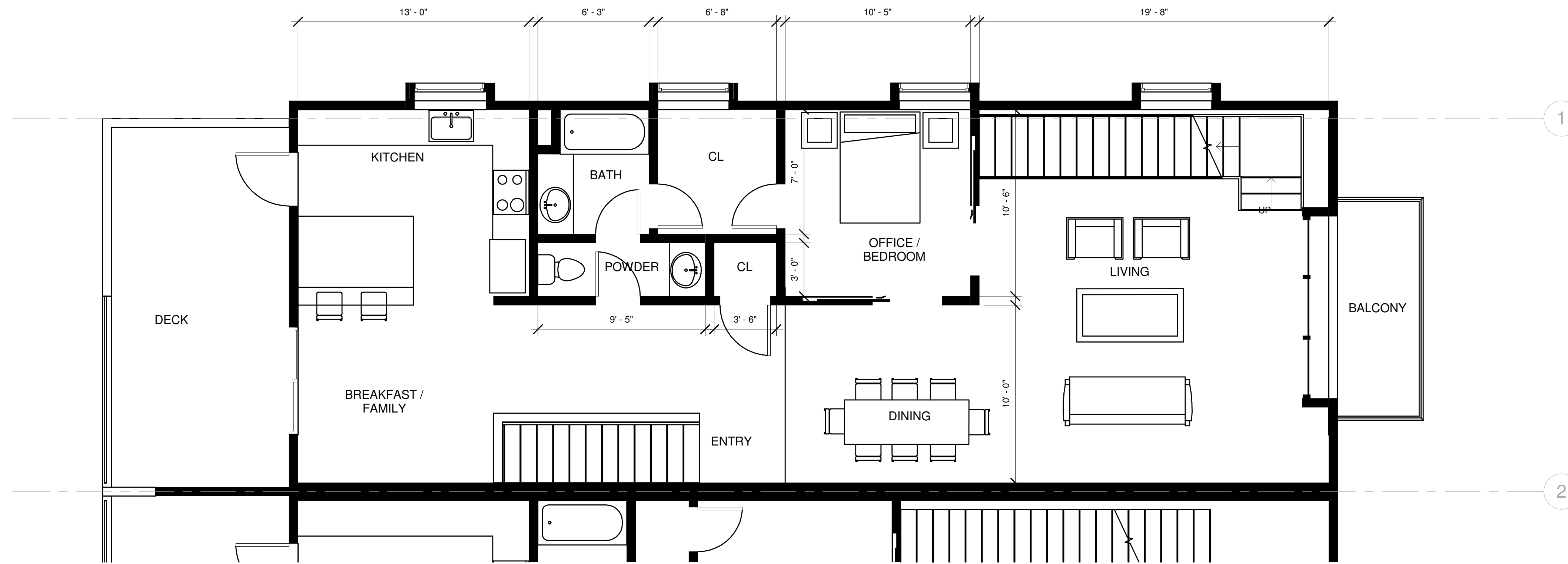
1 UNIT G1 ENLARGED PLAN LEVEL 1 SCALE: 1/4" = 1'-0"
