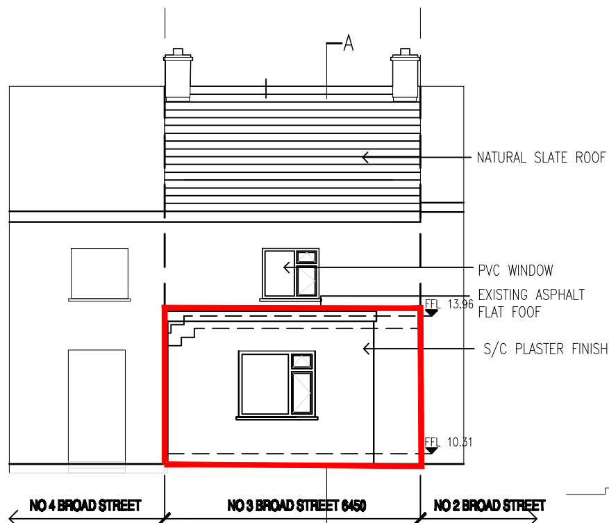
NORTH ELEVATION
