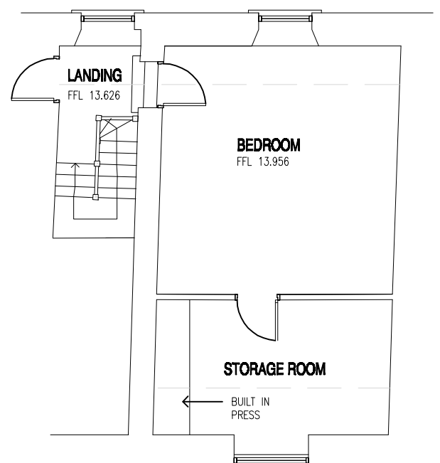
FIRST FLOOR PLAN NO ALTERATIONS
