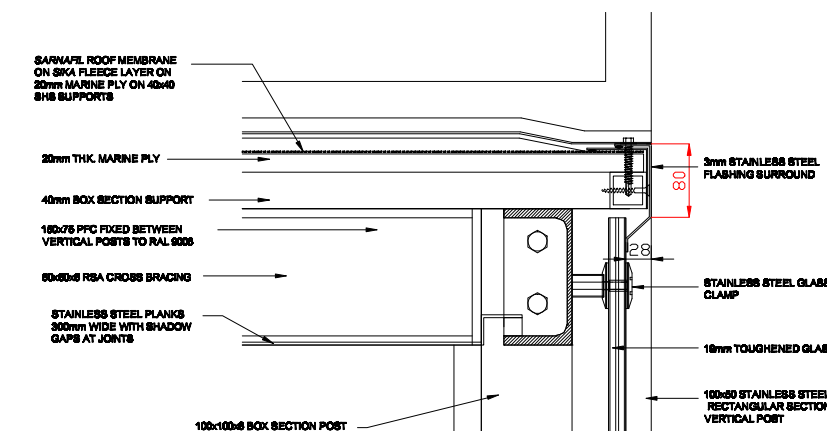
DETAIL C
