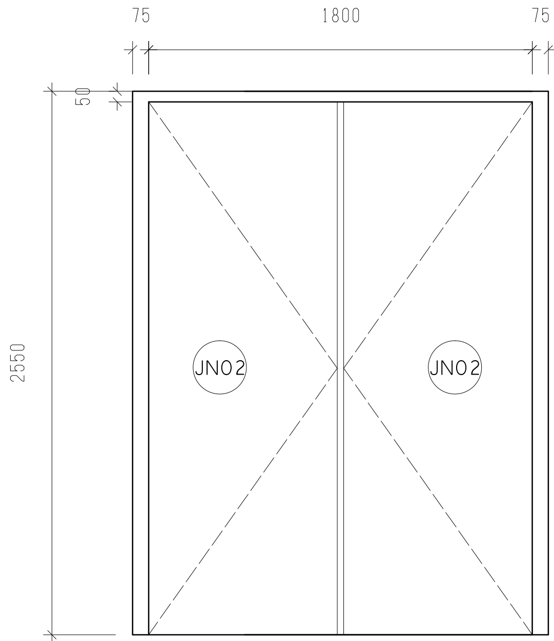
LAUNDRY (door closed)
