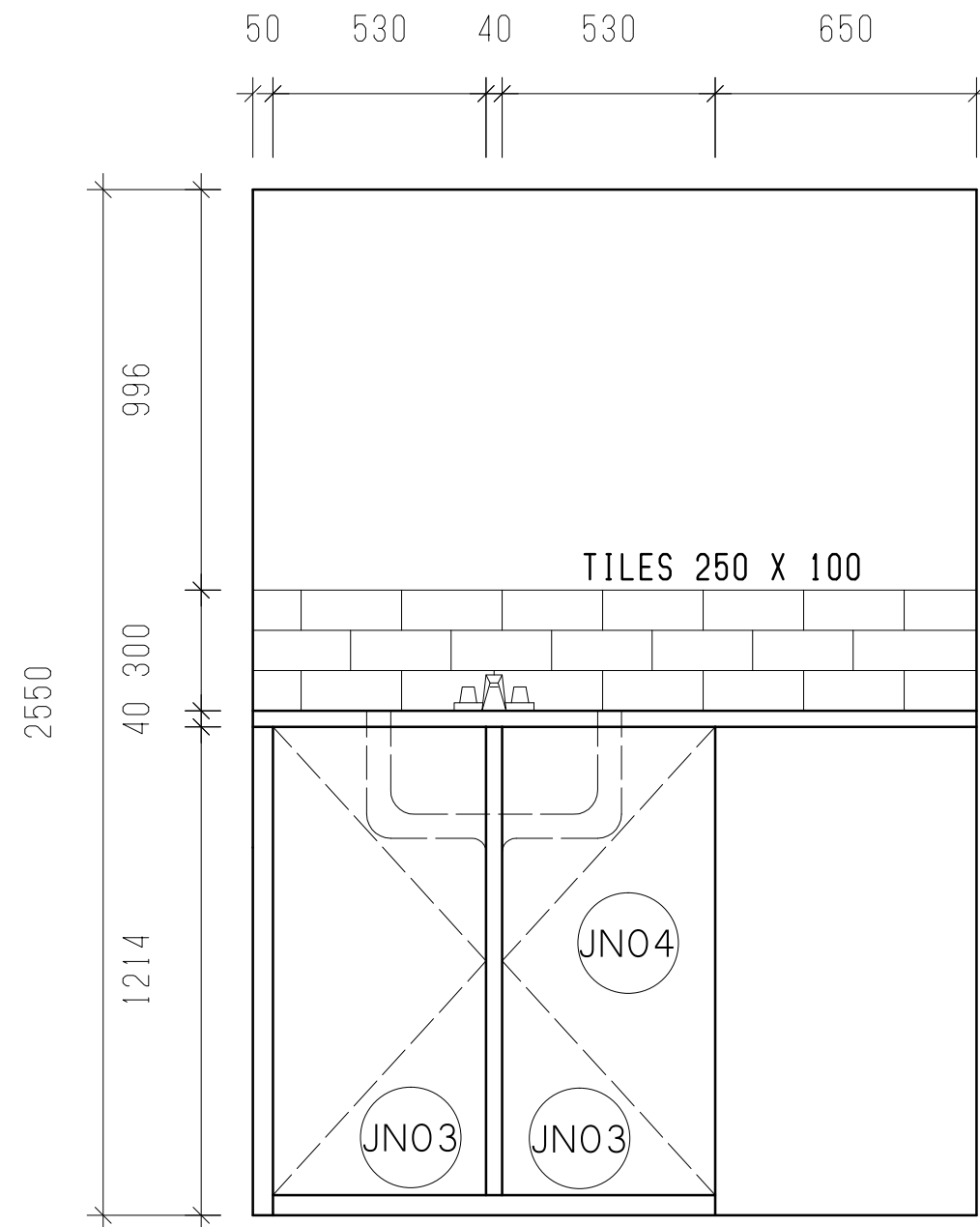
LAUNDRY (doors opened)
