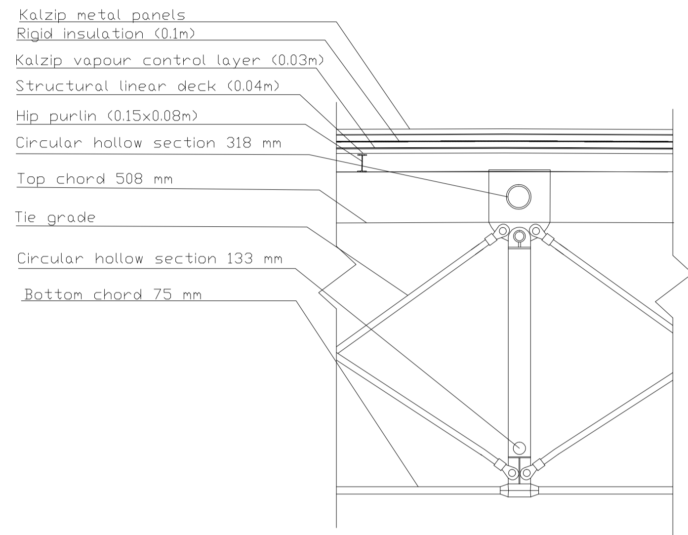
Detail 1 Scale 1:10
