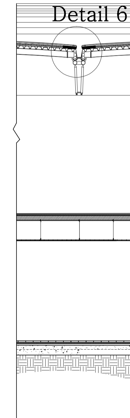
Partial section Scale 1:50 Sheet S3
