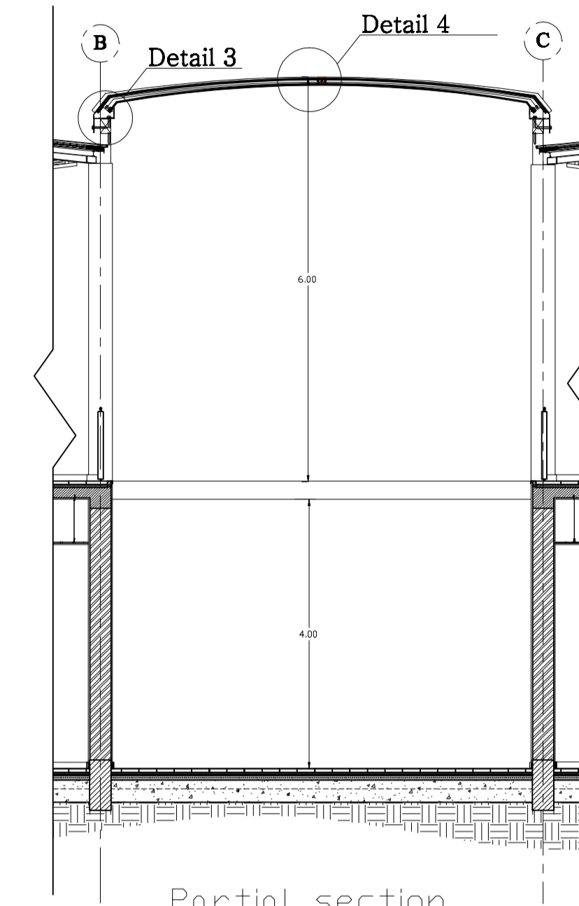
Partial section Scale 1:50 Sheet S3
