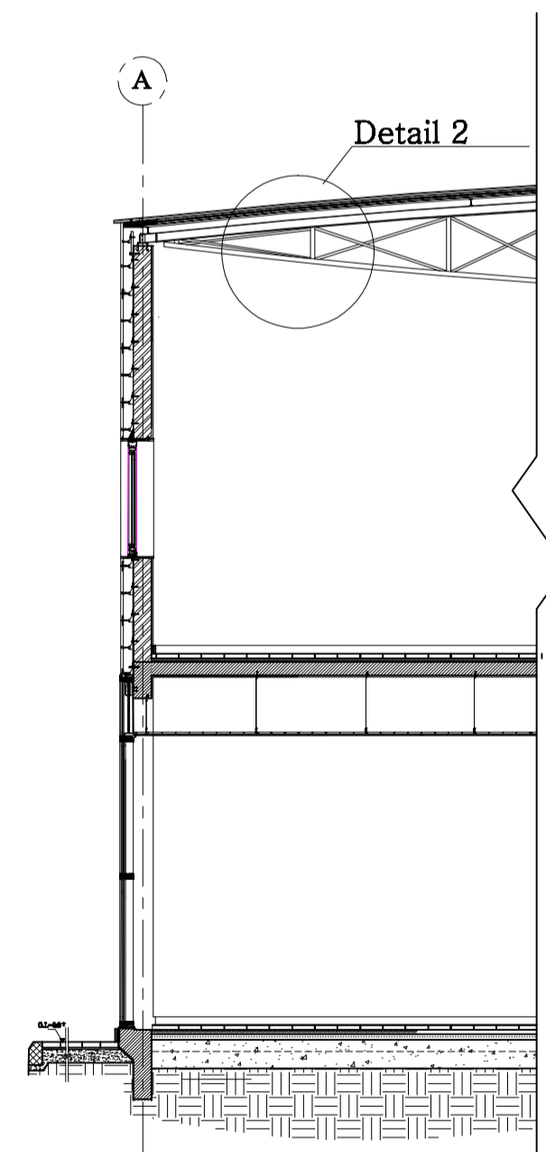
Partial section Scale 1:50 Sheet S3
