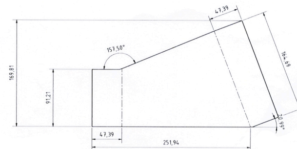
Flat Pattern for MTS_Base_p1&2
