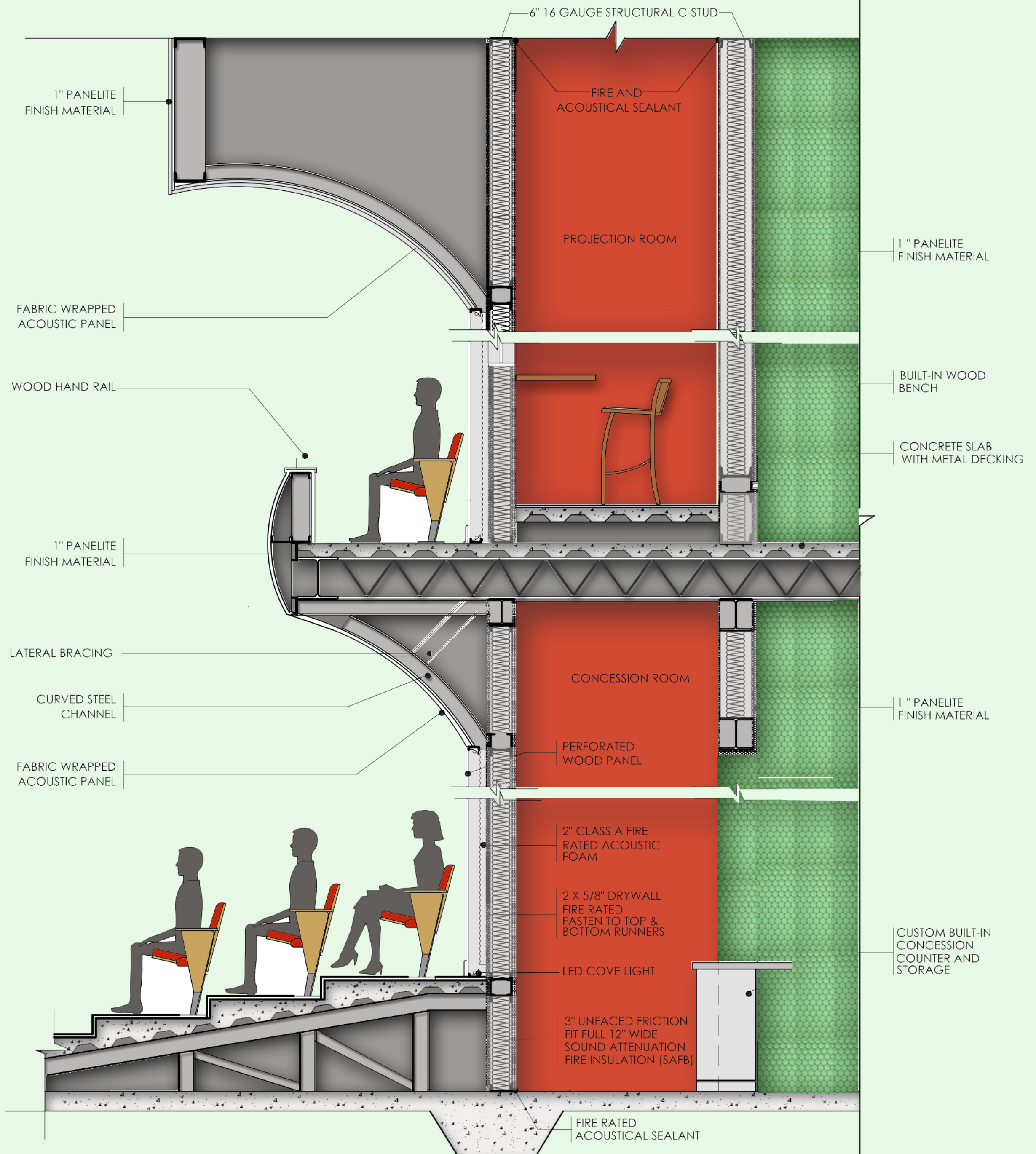
BALCONY SECTION SCALE: 1/2" = 1'-0"
