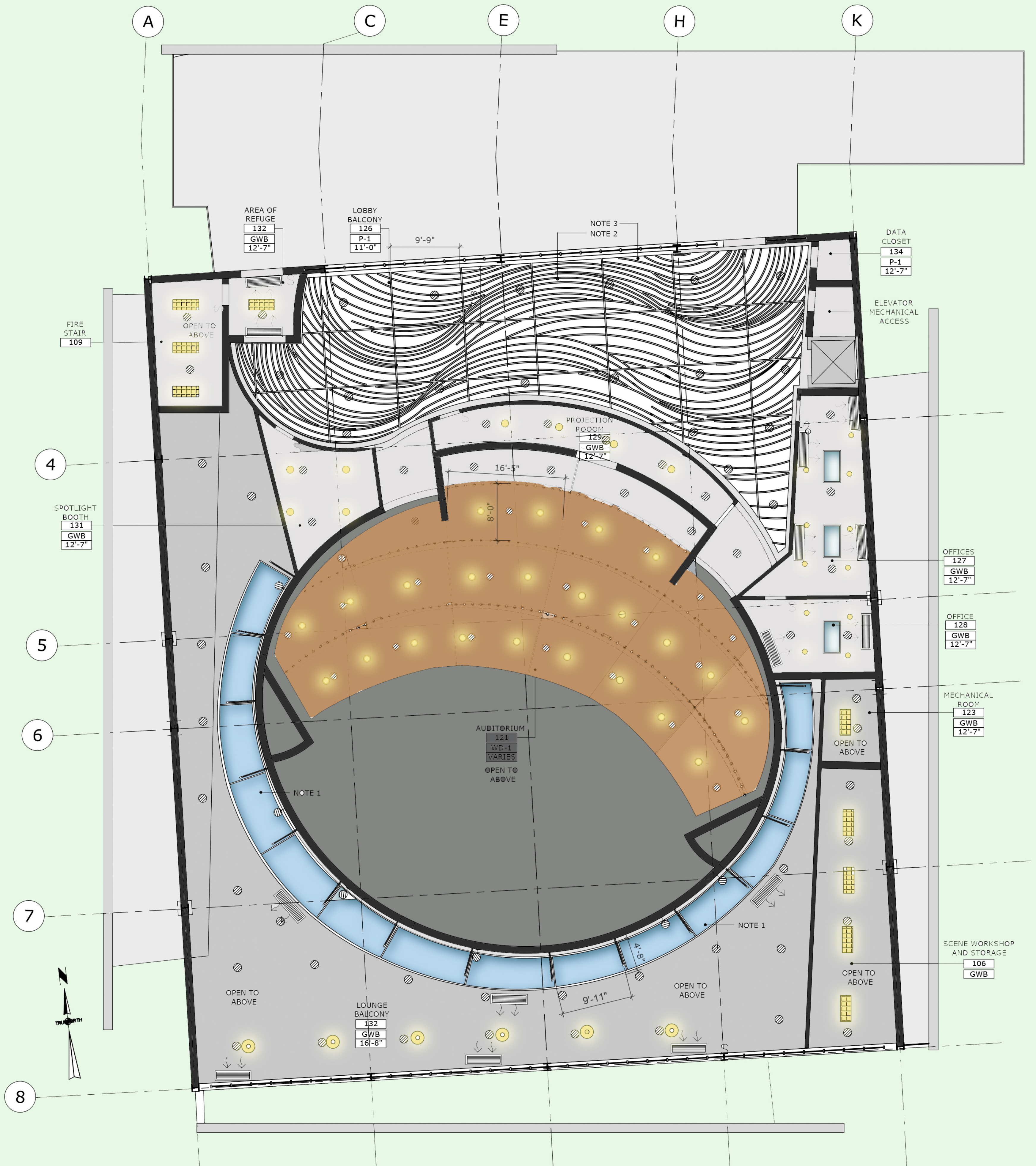
MEZZANINE REFLECTED CEILING PLAN SCALE: 1/8" = 1'-0"
