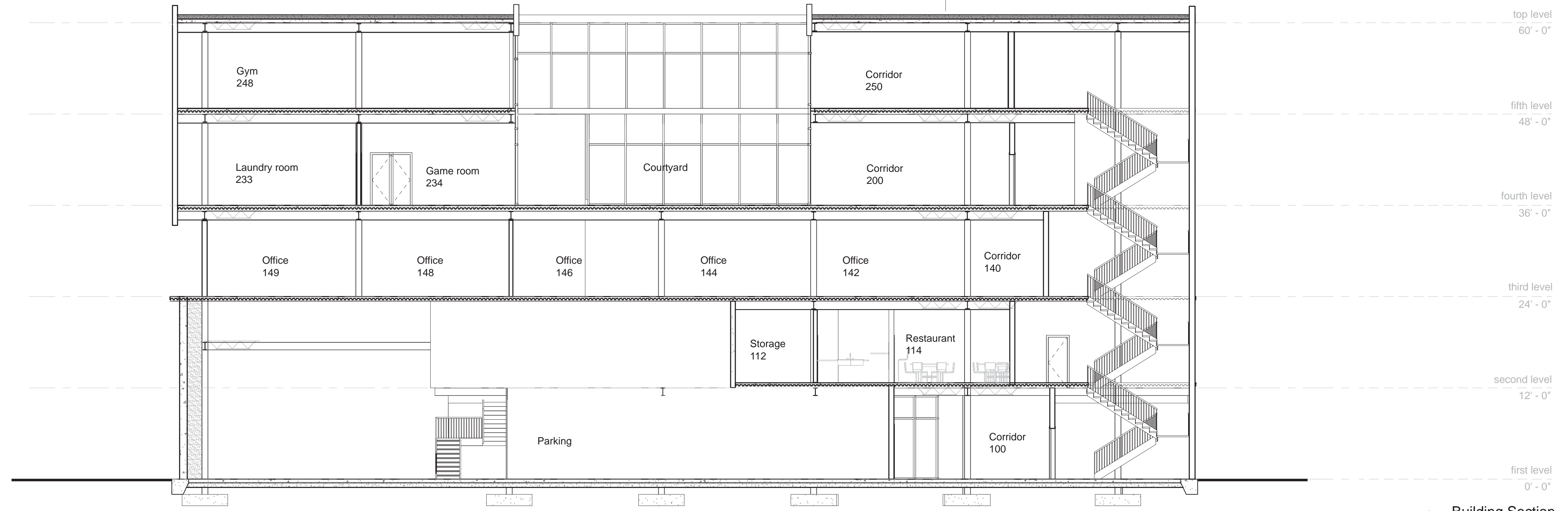
1 Building Section 1/8" = 1'-0"
