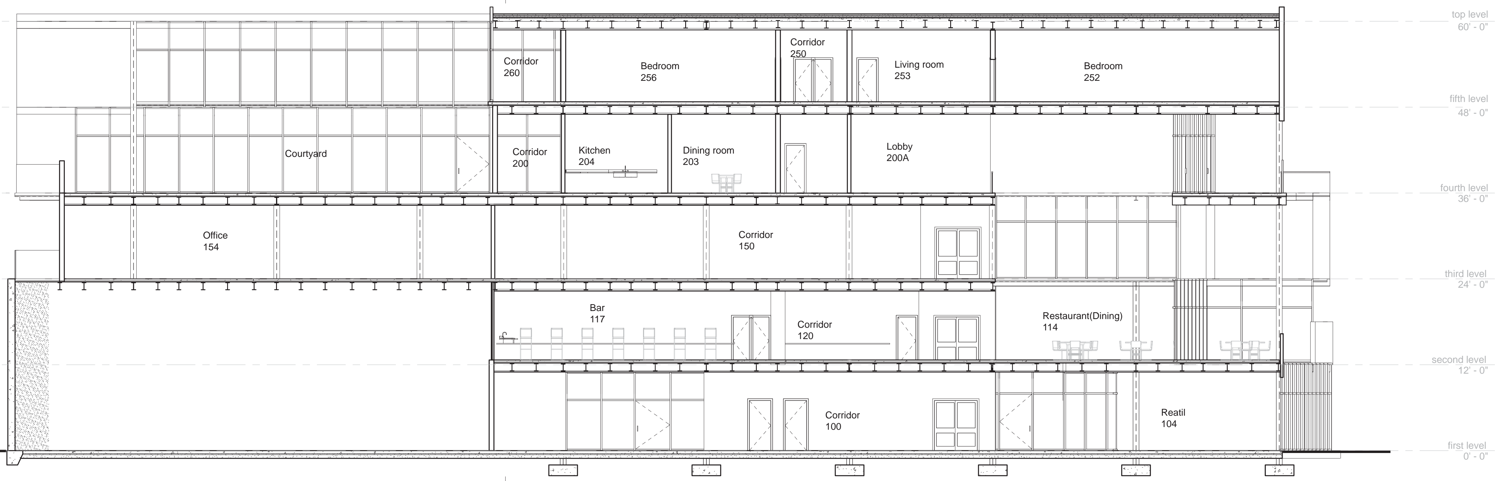
2 Building Section 1/8" = 1'-0"
