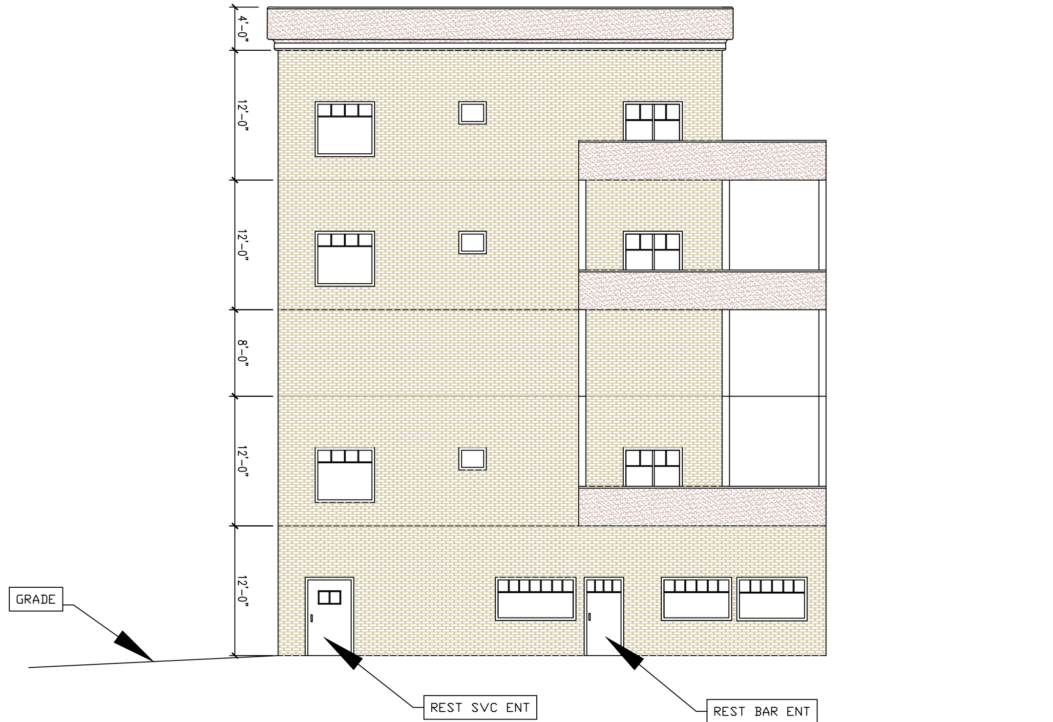
A6 LEFT (WEST) ELEVATION 1/8" = 1'-0"
