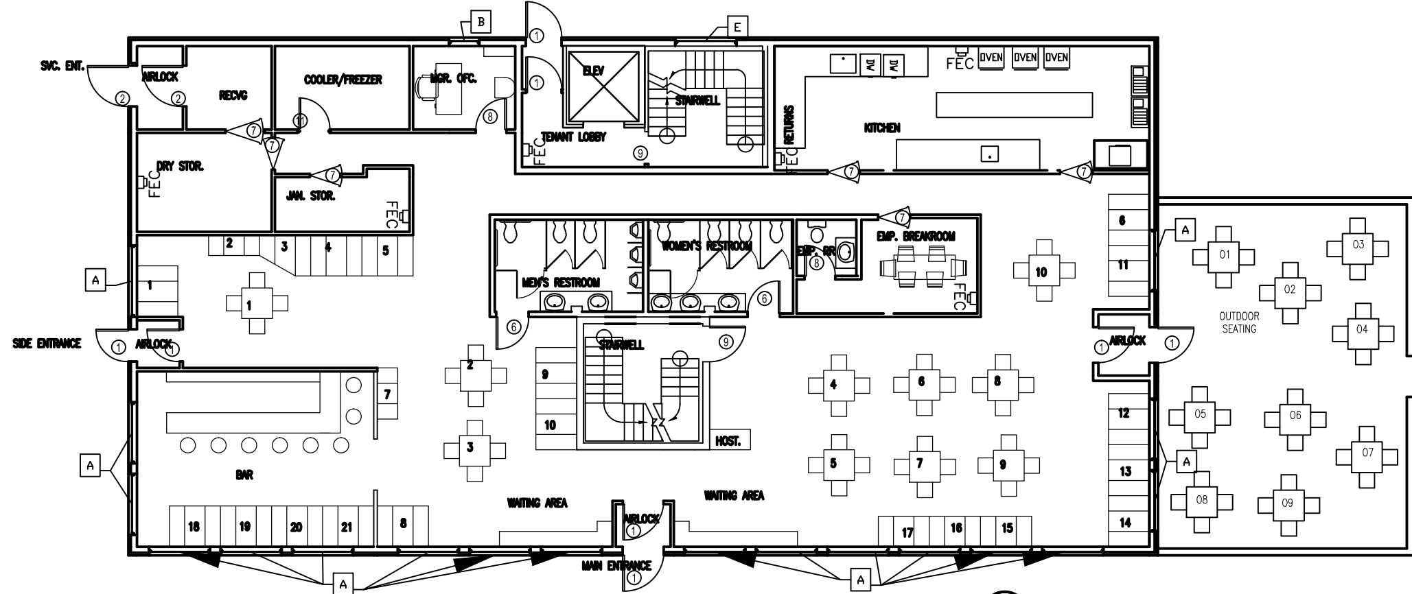
A2- RESTAURANT FLOOR PLAN 1/8" = 1'-0"
