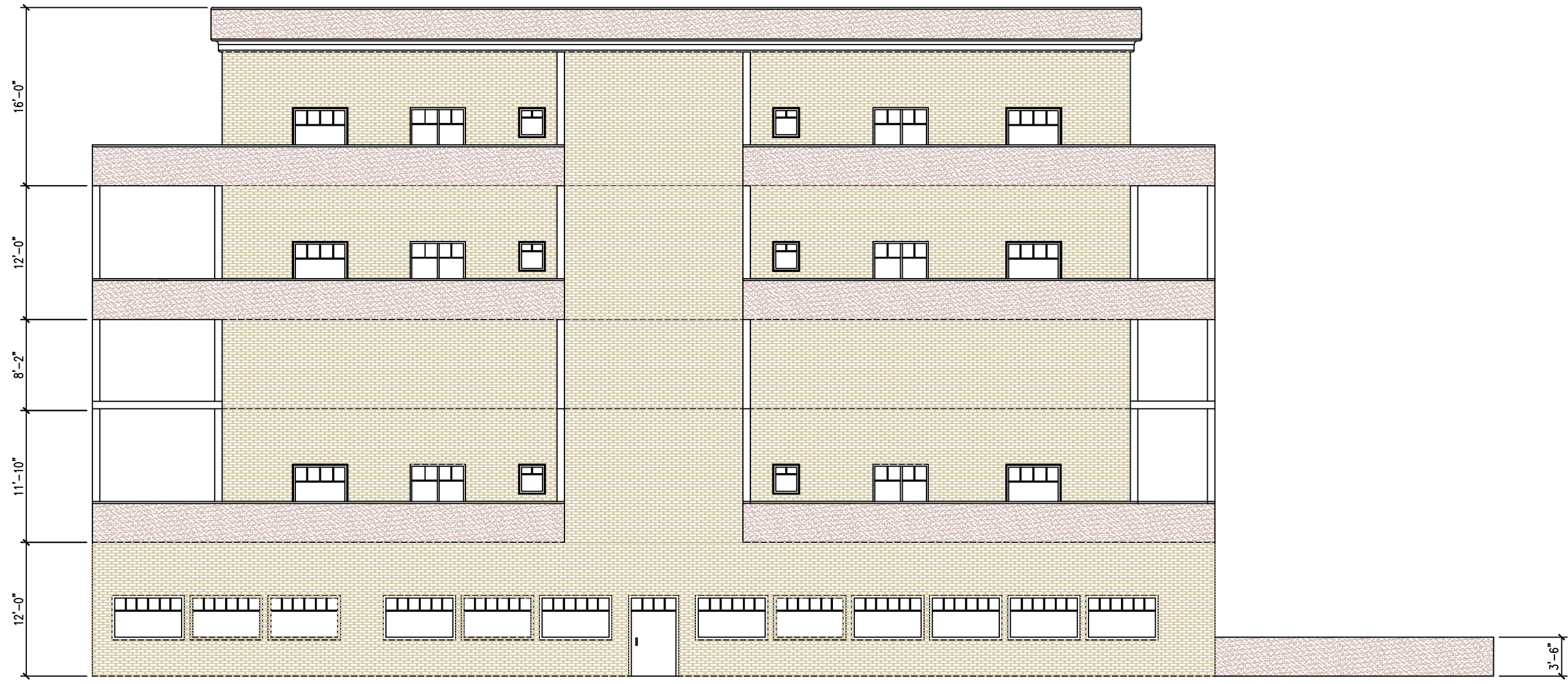
A4 FRONT (SOUTH) ELEVATION 1/8" = 1'-0"
