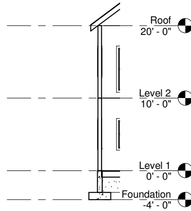
① Section 1 1/8" = 1'-0"
