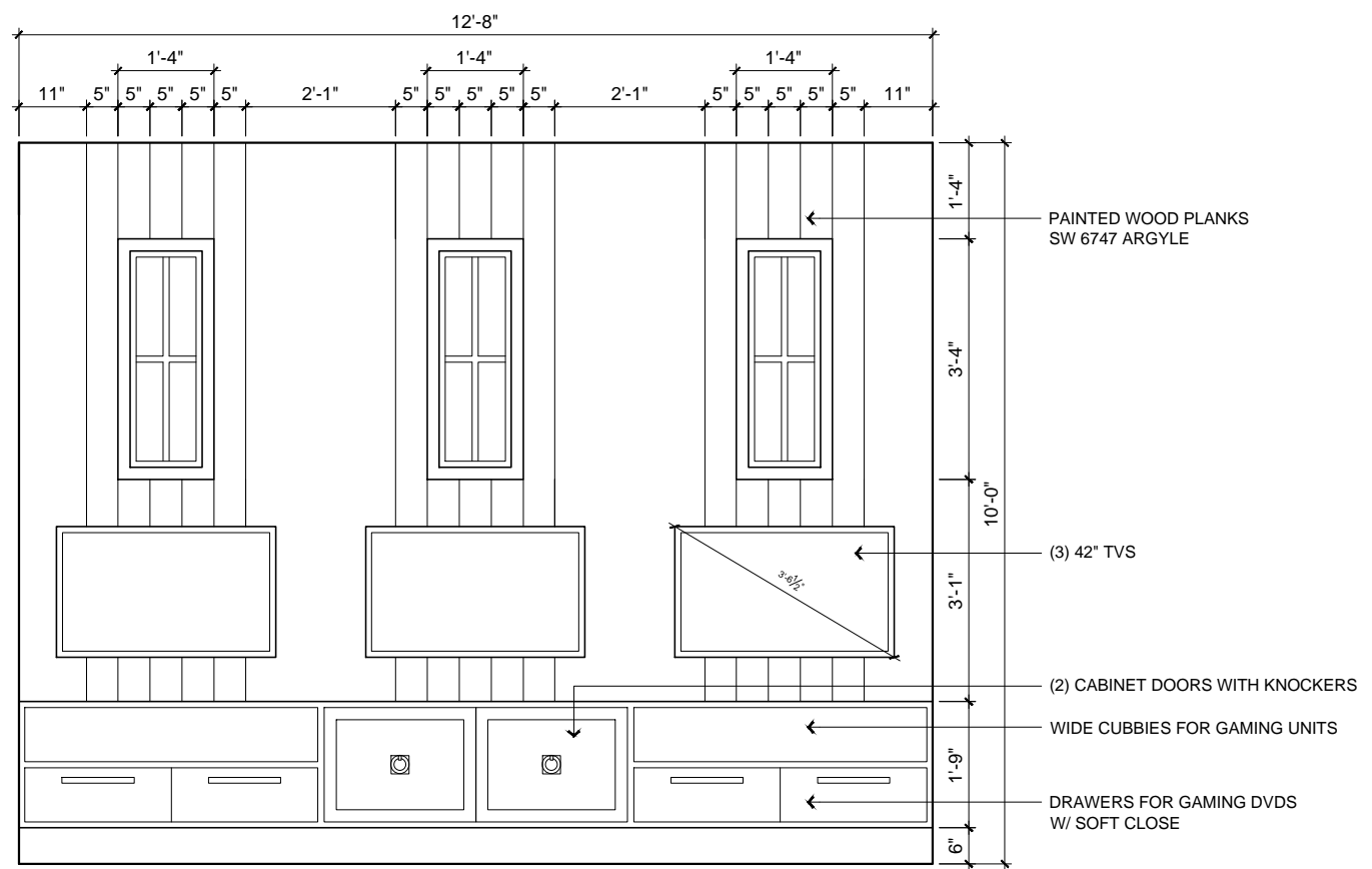
HAYDEN'S BUILT-IN ELEVATION SCALE: 3/8" = 1' - 0" BUILT-IN TO BE STAINED TO MATCH BATH CABINETS. PLEASE SEE SAMPLE OR INSTALLED CABINETS FOR REFERENCE.
