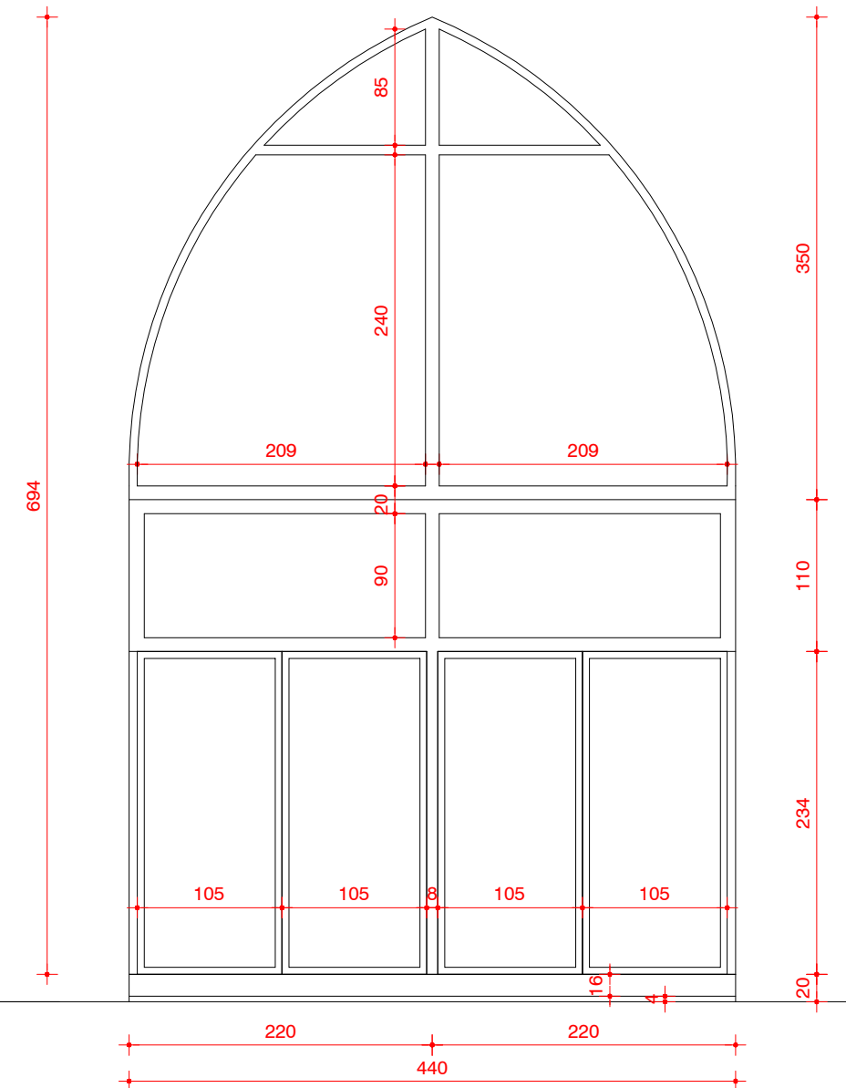
5 FIXED GLASSES (D) 2 OF THEM ARE WITH PRINT FILM (D')
