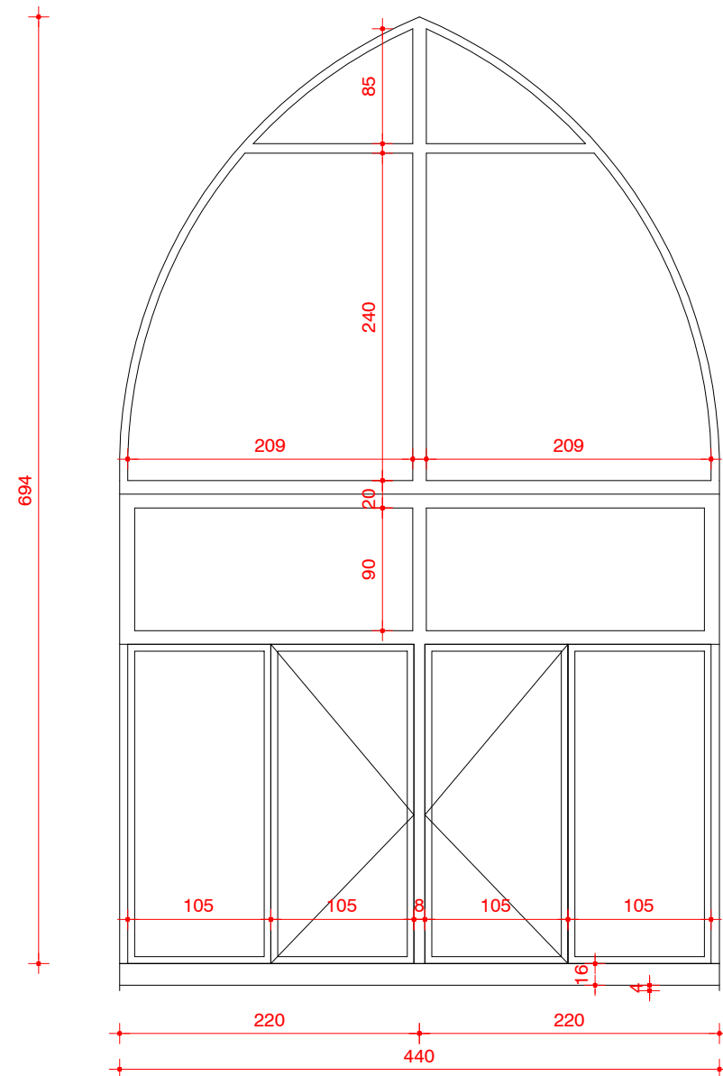
1 SET ENTRANCE OPENED GLASS DOOR (A)
