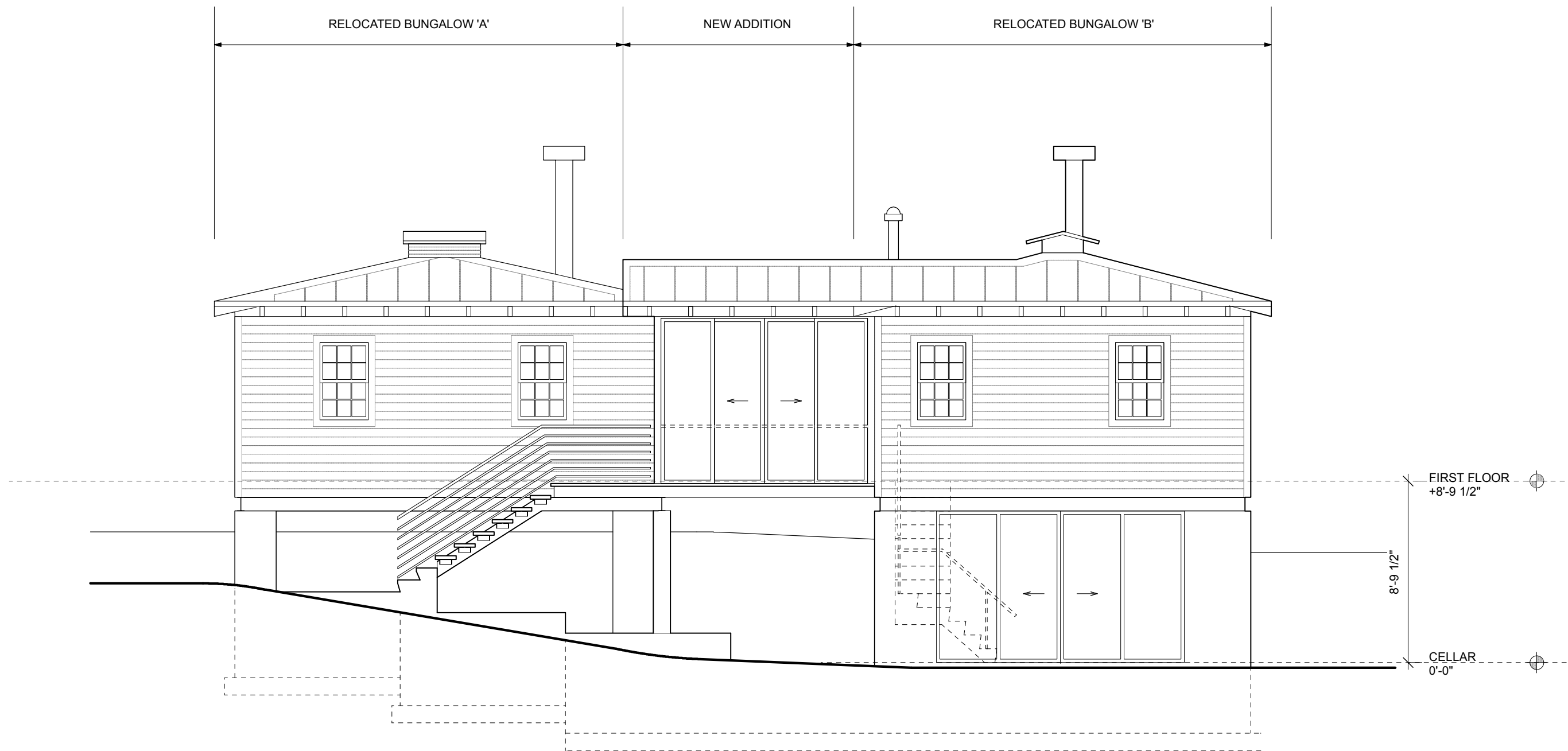
1 ELEVATION @ SOUTH A2.1 SCALE 3/16" = 1'-0"
