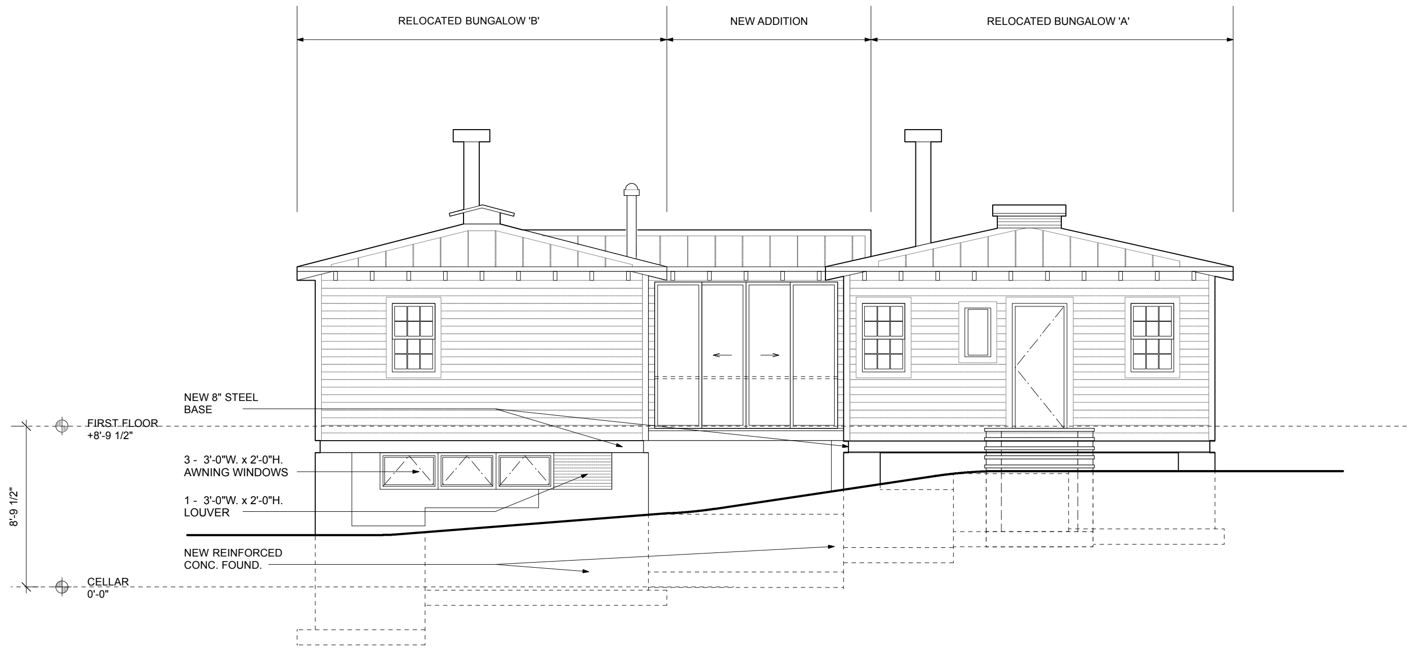
1 ELEVATION @ NORTH A2.2 SCALE 3/16" = 1'-0"
