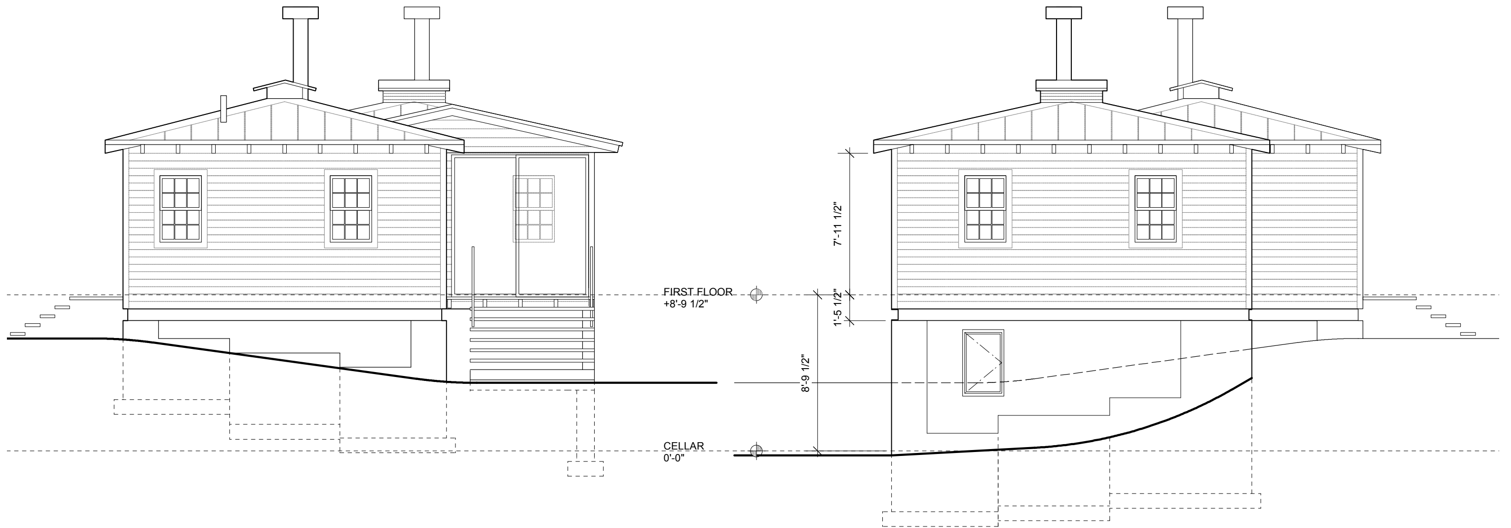
2 ELEVATION @ WEST A2.0 SCALE 3/16" = 1'-0"
