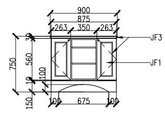
J5 FRONT VIEW SCALE 1:50m
