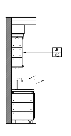
SECTION A SCALE 1:50m
