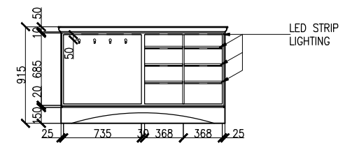
J1 W/O DOORS FRONT VIEW SCALE 1:50m
