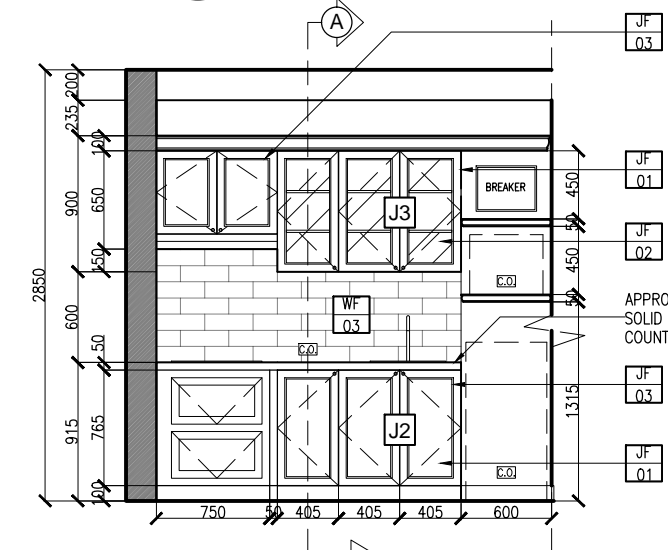
J2 & J3 FRONT VIEW SCALE 1:50m
