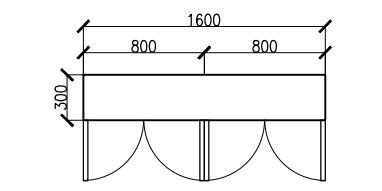
J1 TOP VIEW SCALE 1:50m
