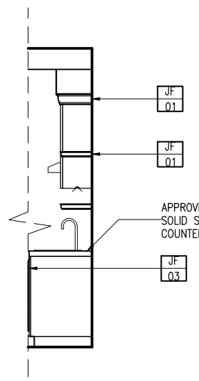
J2 & J3 SIDE VIEW SCALE 1:50m
