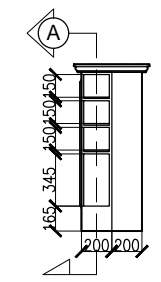
J4 SIDE VIEW SCALE 1:50m
