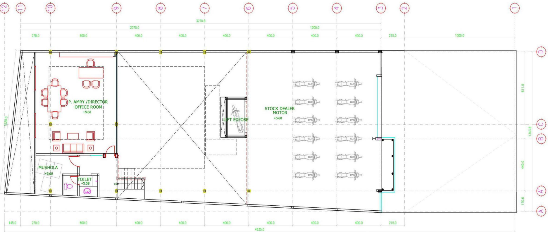
FLOOR PLAN 3rd - SCALE 1 : 200
