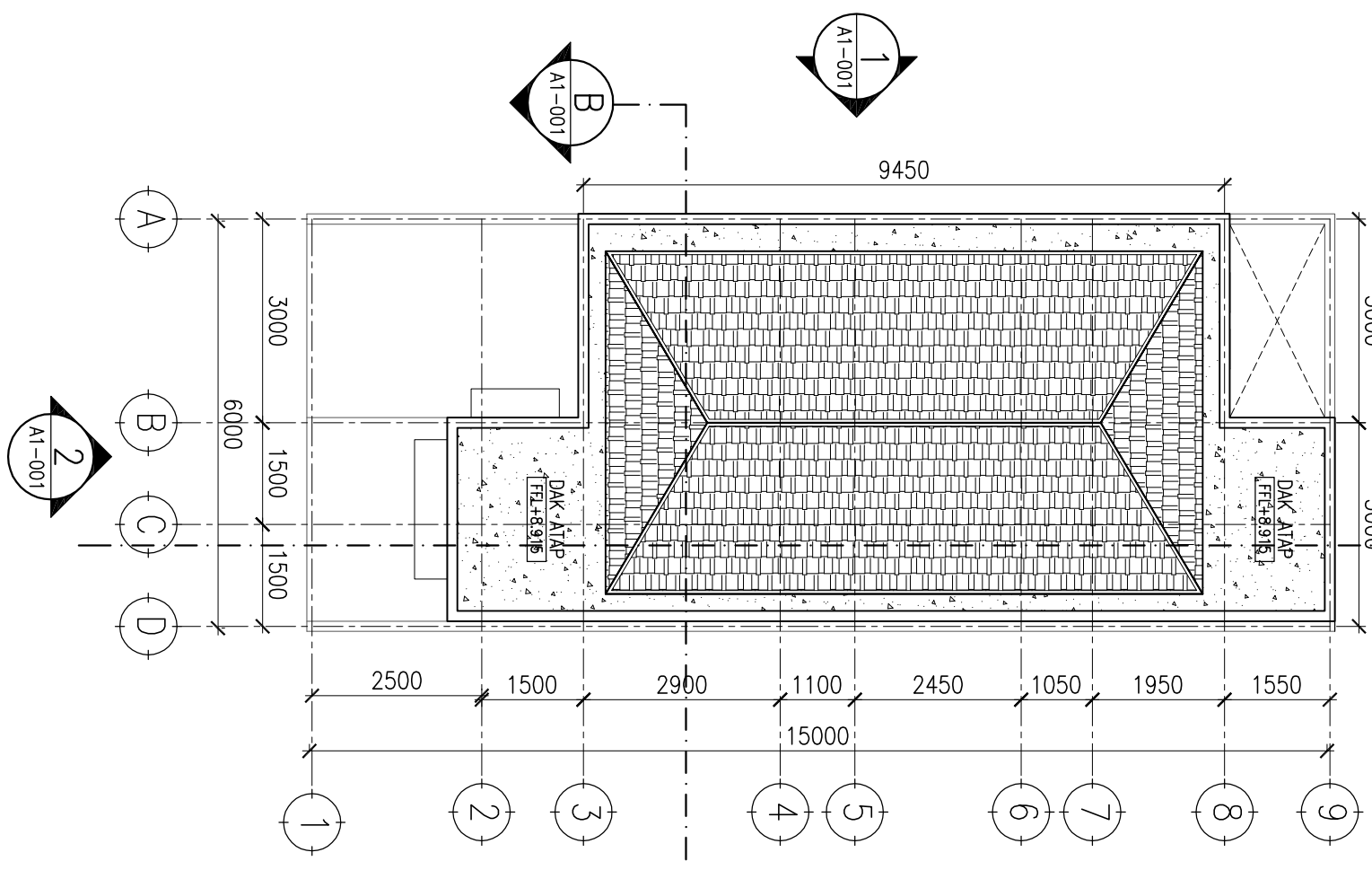
1 DENAH ATAP A1-001 SCALE 1 : 100
