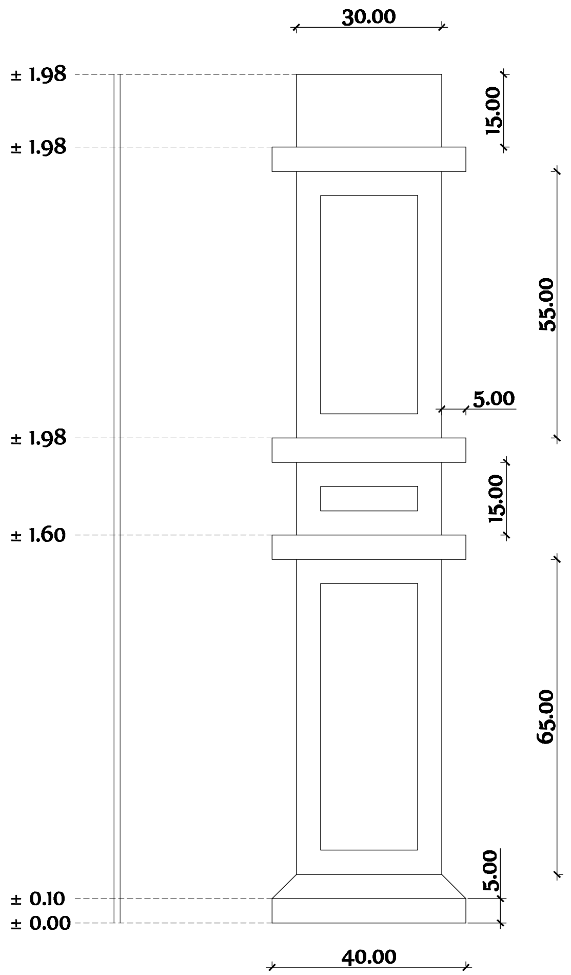
Detail Tipe 1
