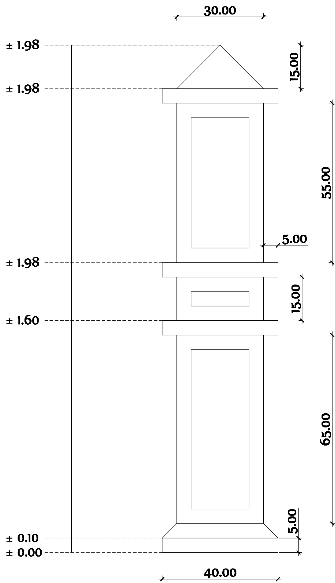
Detail Tipe 1
