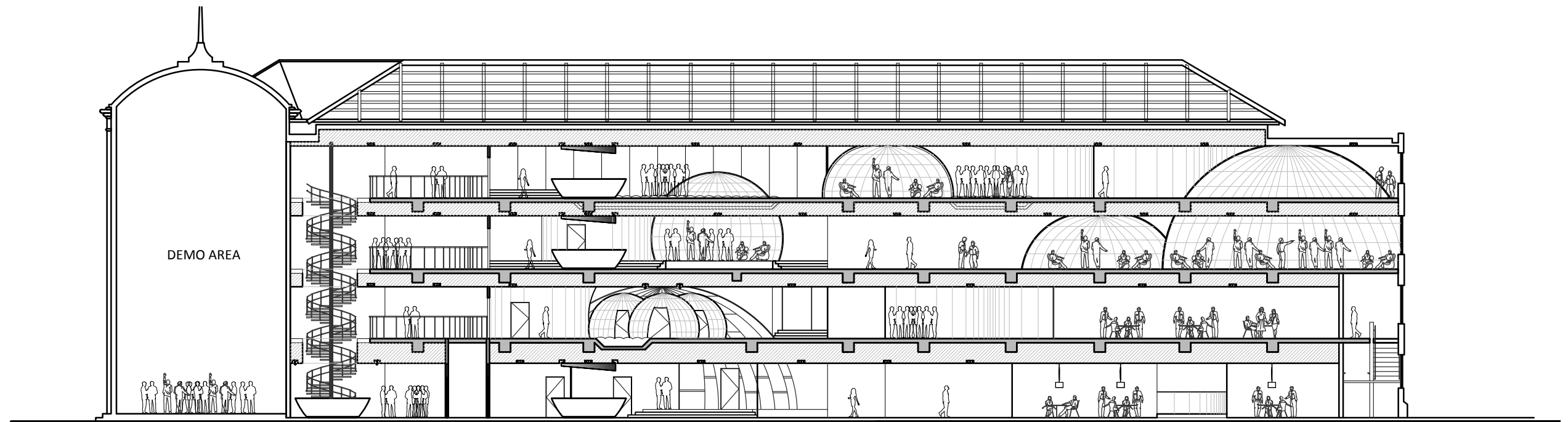
SECTION A 1:250
