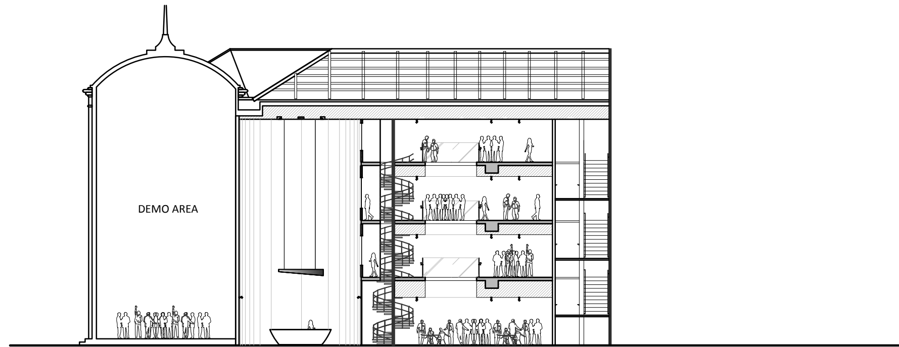
SECTION B 1:250
