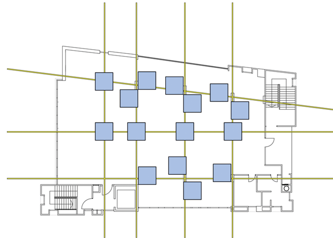
Placing Individual Pods around column
