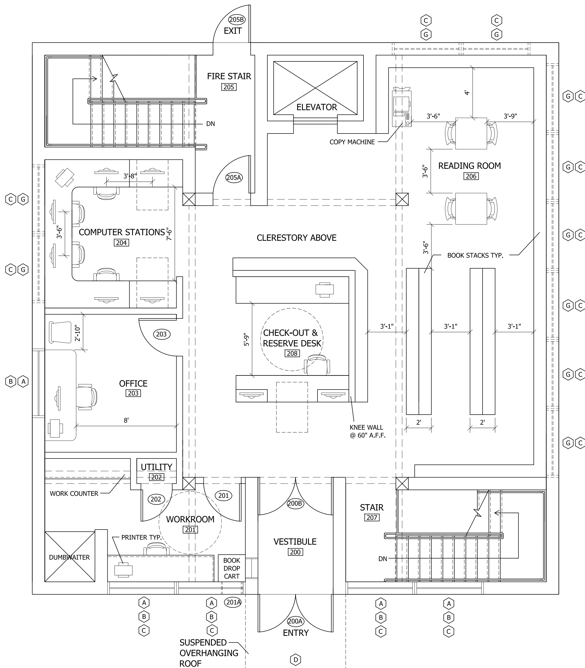
1 FIRST FLOOR FURNITURE FLOOR PLAN SCALE: 1/4" = 1'-0"
