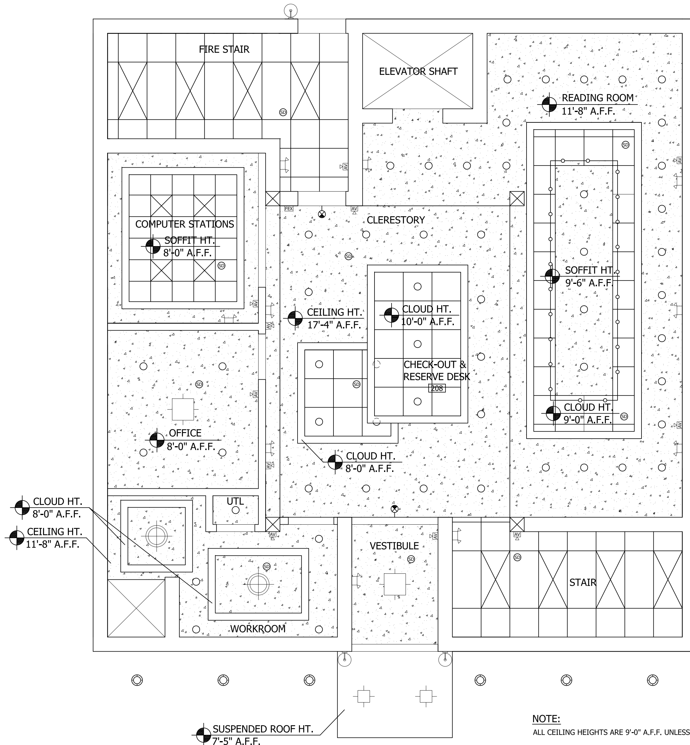
1 FIRST FLOOR REFLECTED CEILING PLAN SCALE: 1/4" = 1'-0"
