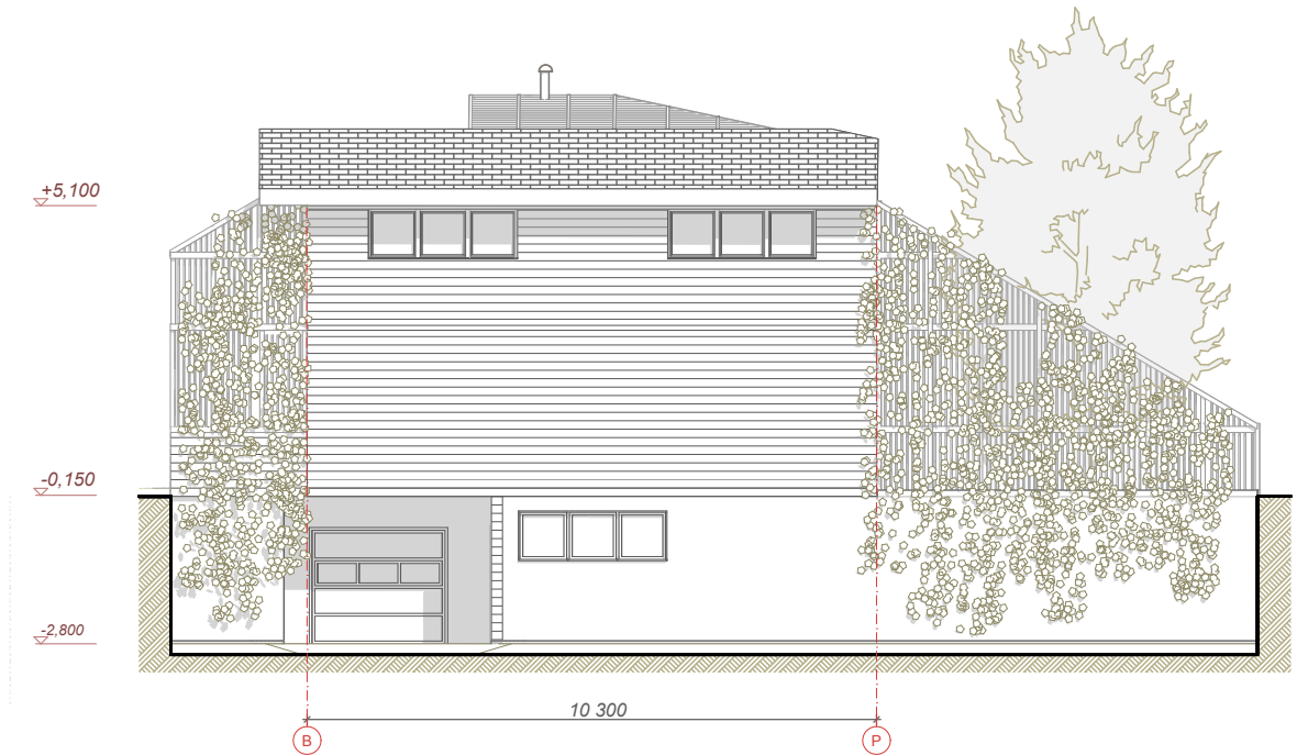
North west facade
