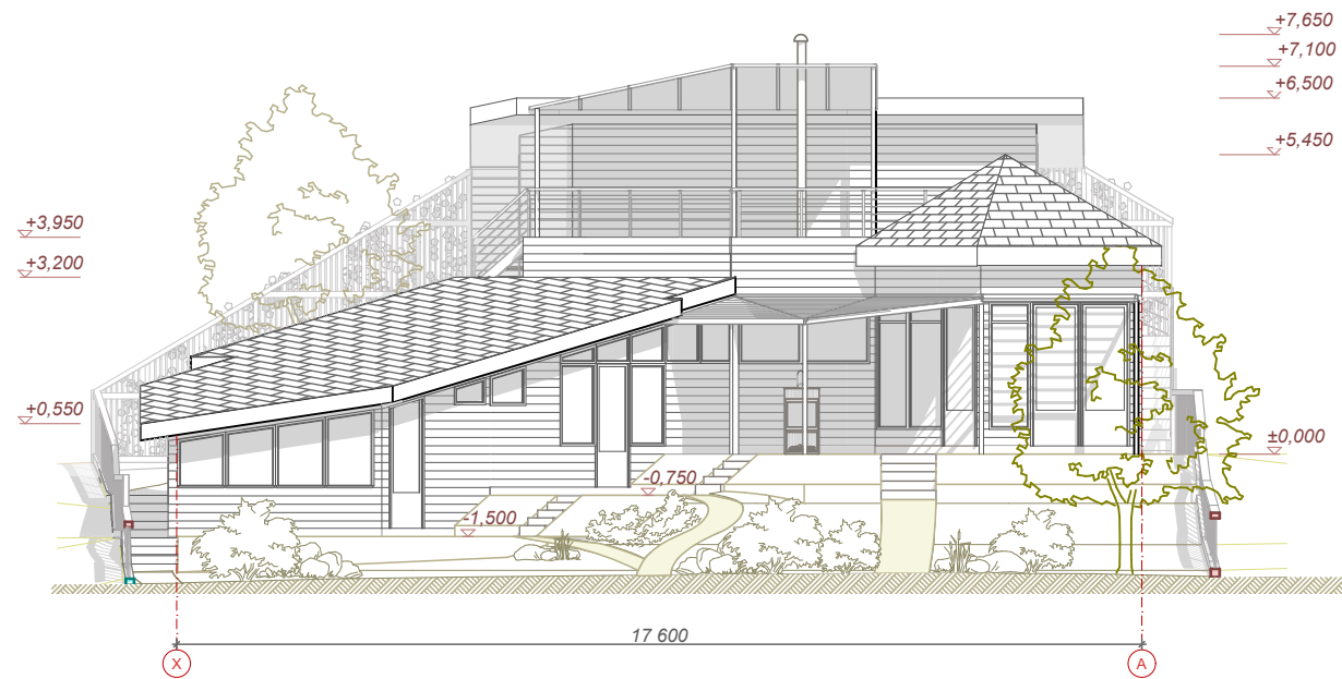
South east facade
