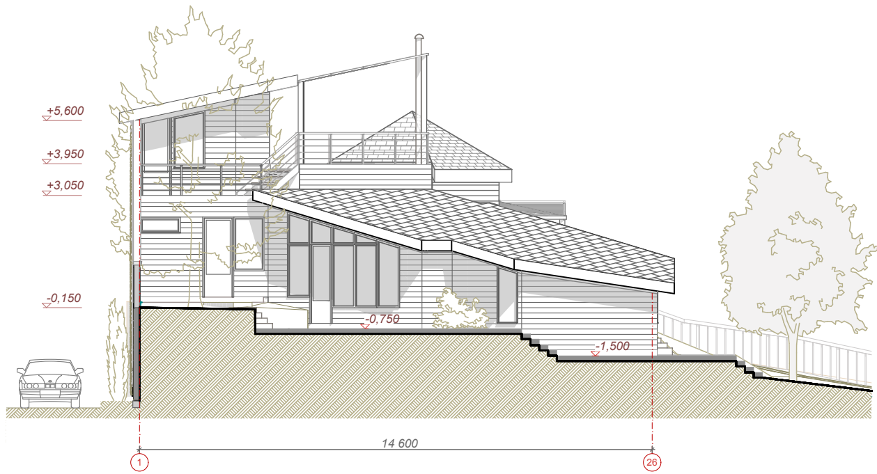
South west facade
