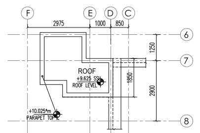
UPPER ROOF PLAN SCALE 1:100
