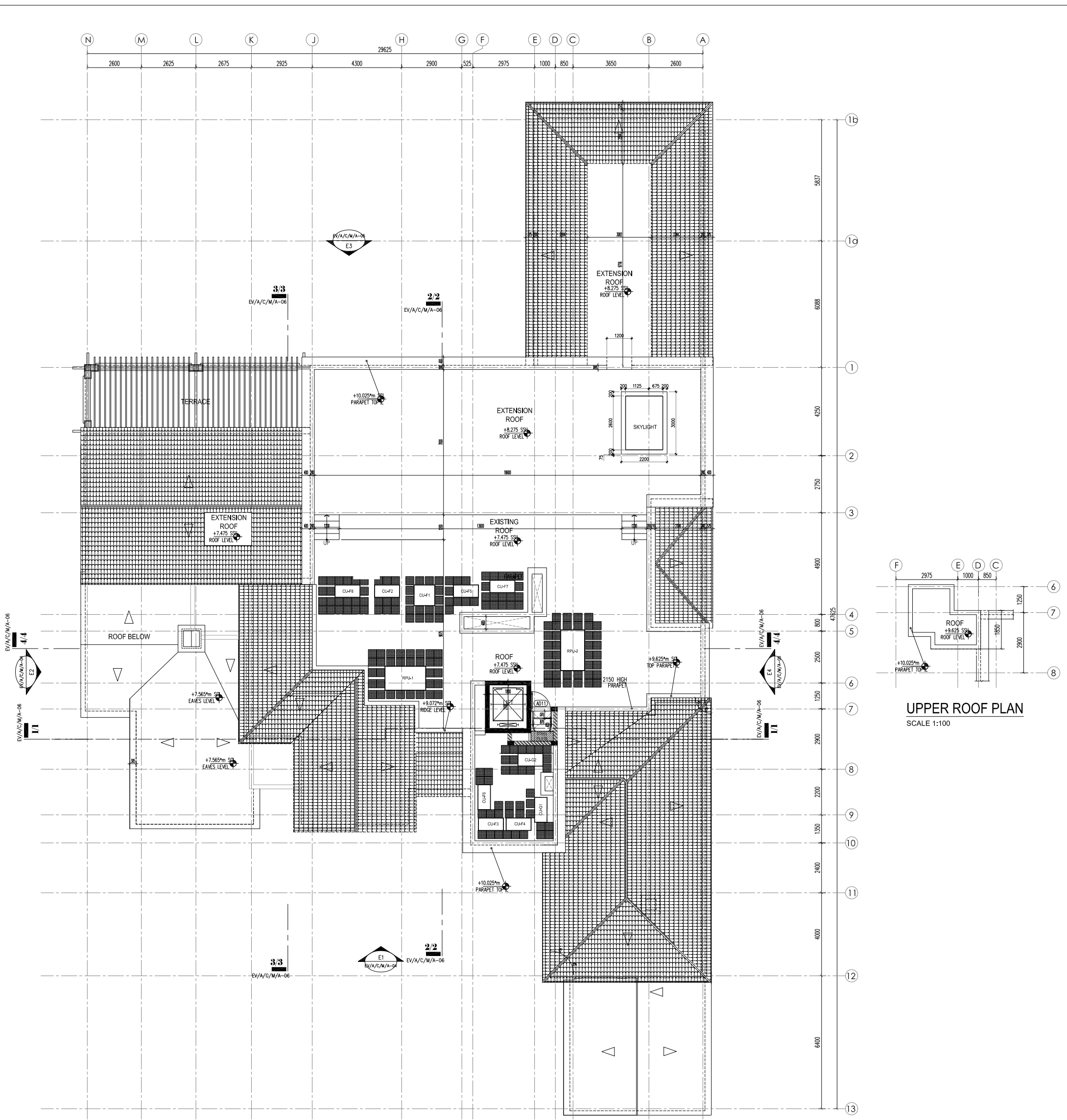
ROOF AND UPPER ROOF PLAN
