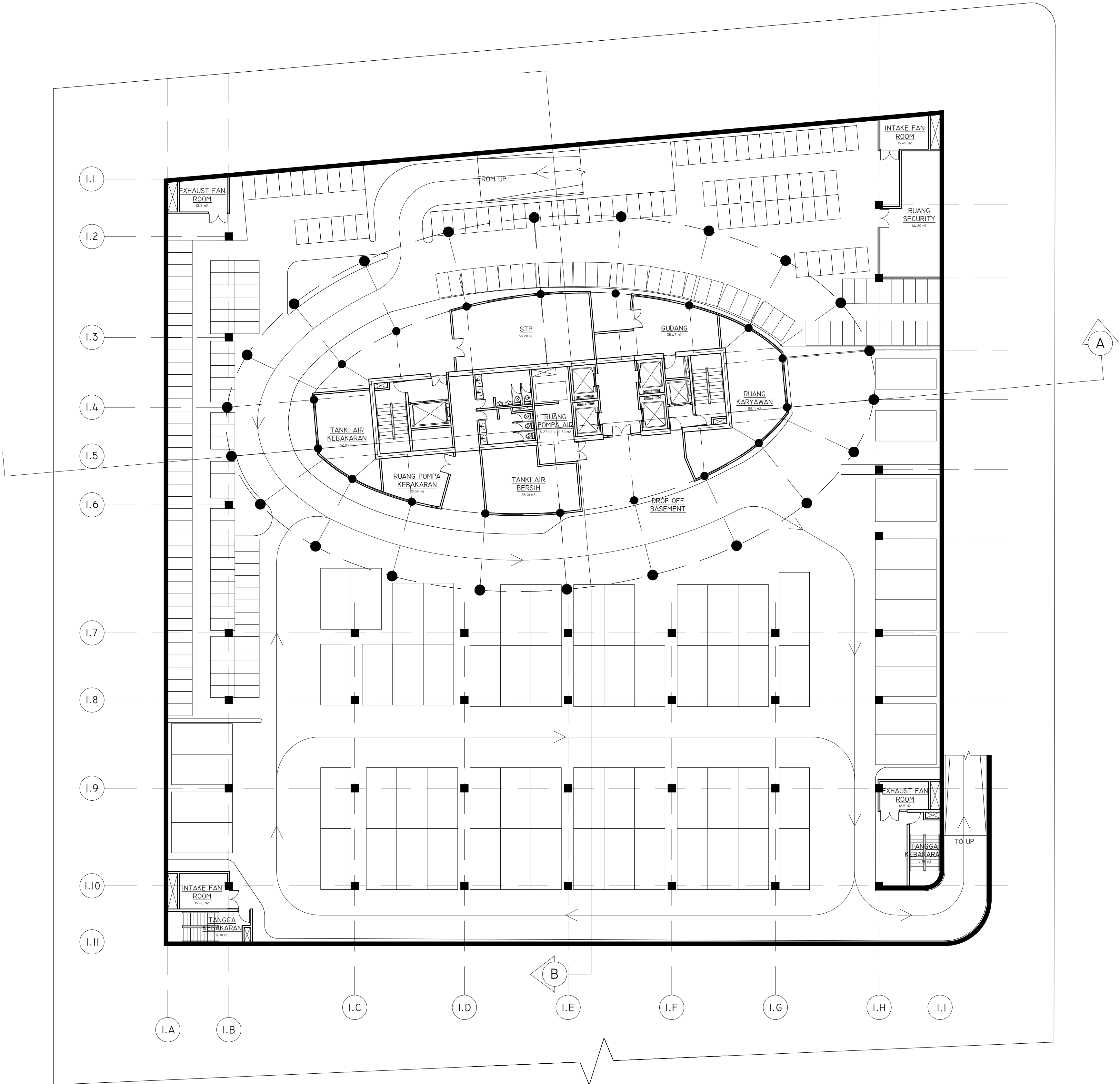
DENAH BASEMENT LANTAI 3 SKALA 1 : 200
