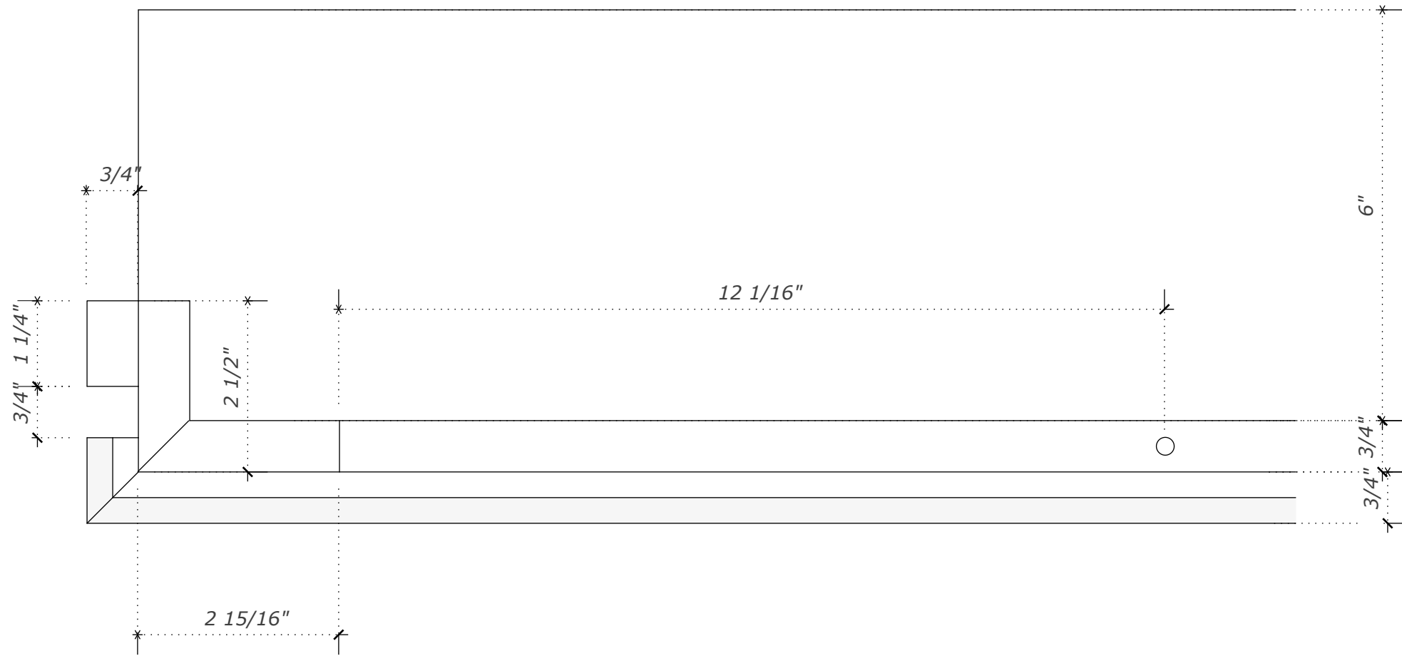
TOP Cross section
