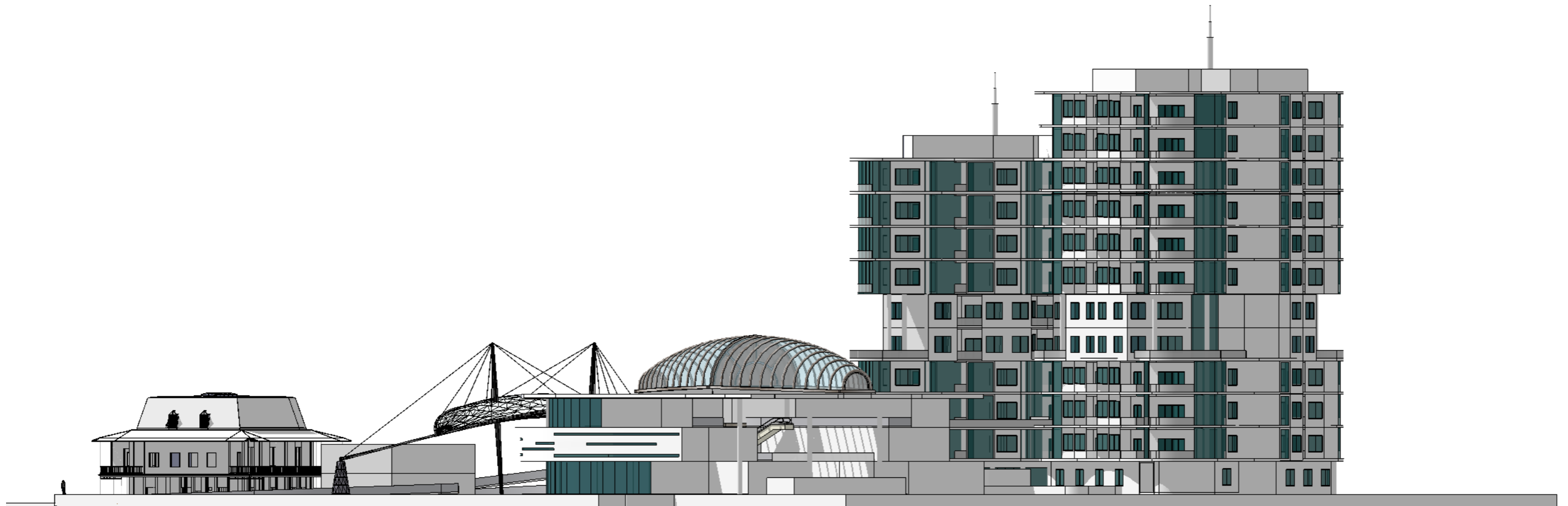
TAMPAK SAMPING KANAN SKALA 1:500
