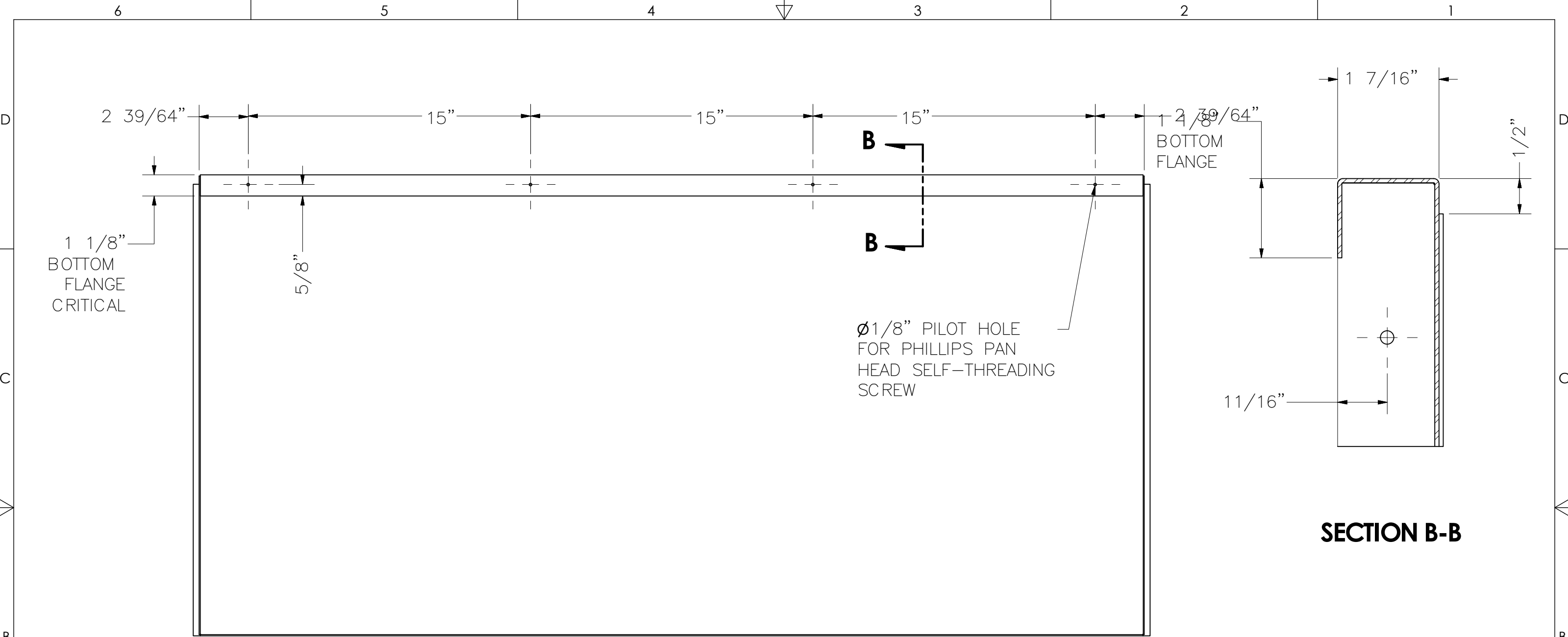
BOTTOM VIEW
