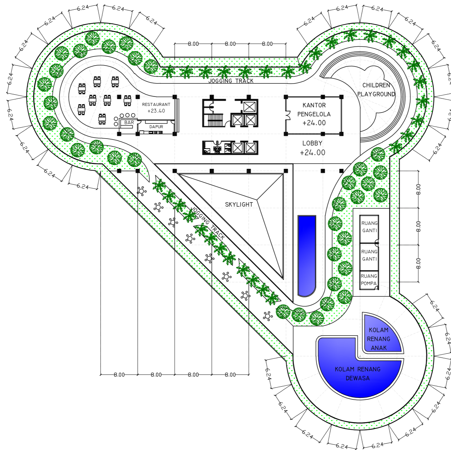
DENAH ROOFTOP SKALA 1:500
