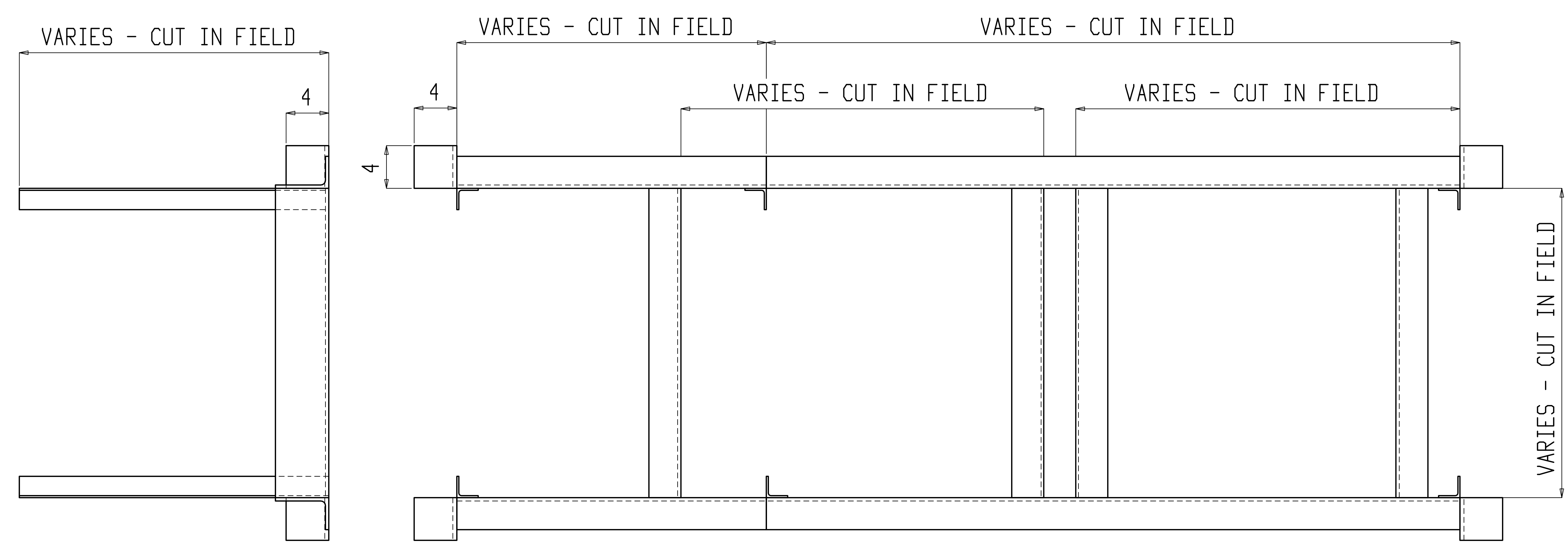
TYPICAL RTU FRAME - VARIES - CUT IN FIELD
