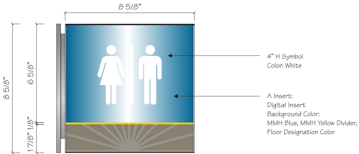
(1) A Insert = 8 5/8" x 8 1/2" Module 6.0 DPM - Sign Type Q - Double Perpendicular Mounted Mount Painted Metallic Silver to Match
