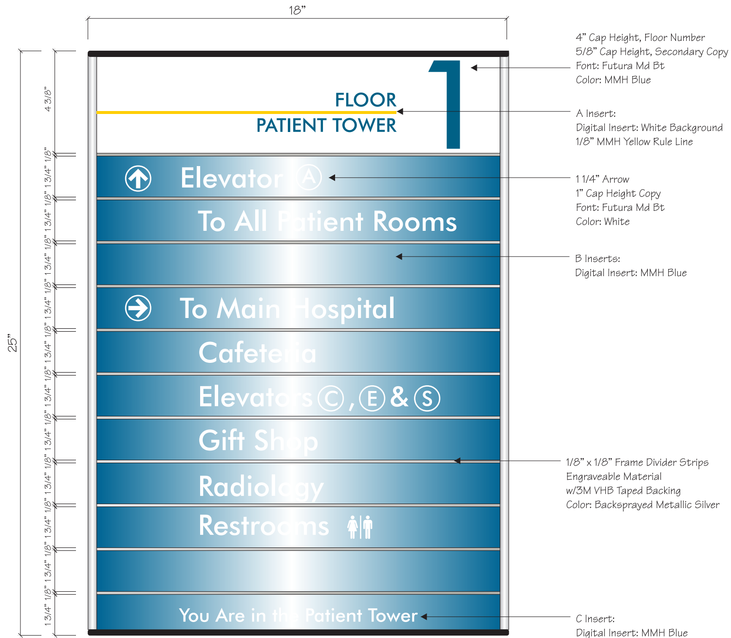
(1) A Insert = 1 3/4" x 17 7/8" (10) B Insert = 1 3/4" x 17 7/8" (1) C Insert = 1 3/4" x 17 7/8"
