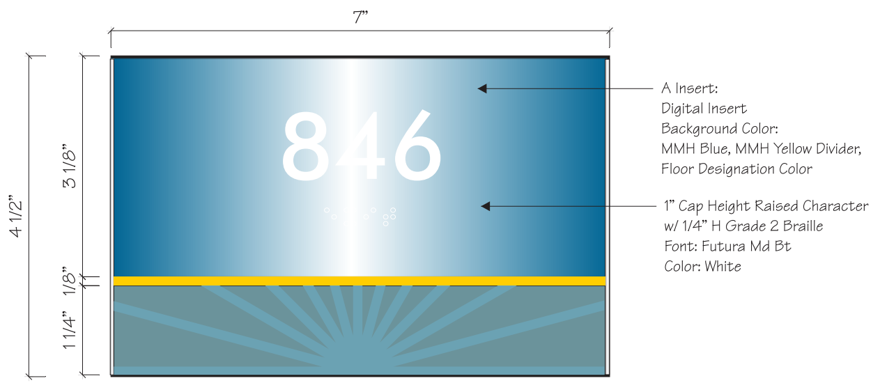
(1) A Insert = 4 1/2" x 6 7/8" Module 3.7 ID - Sign Type C - Patient Room ID
