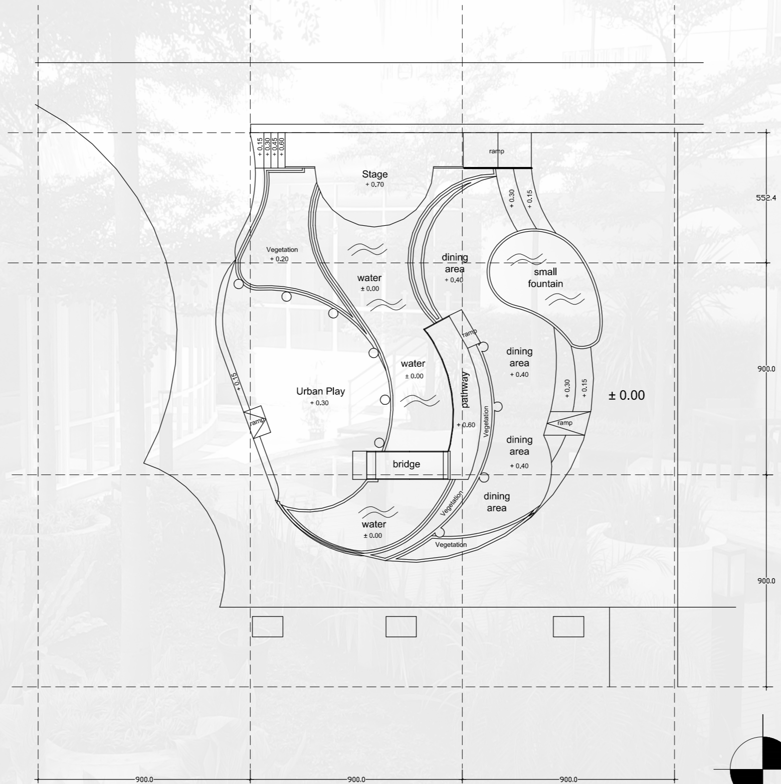
DENAH TAMAN 1:16
