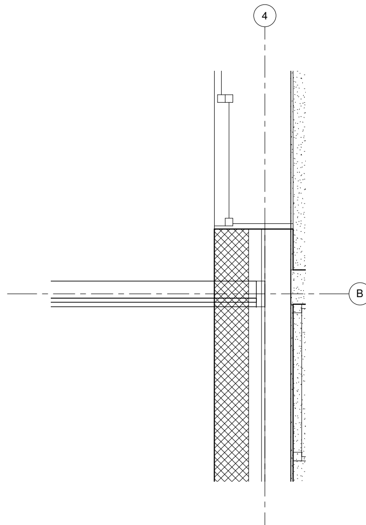
2 Detail at Wall Intersection 1 : 10
