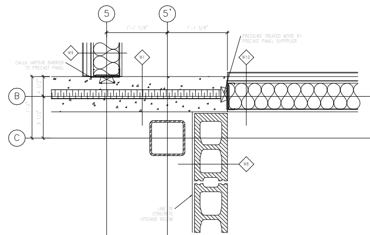
1 Wall Roof Intersection 1 : 10
