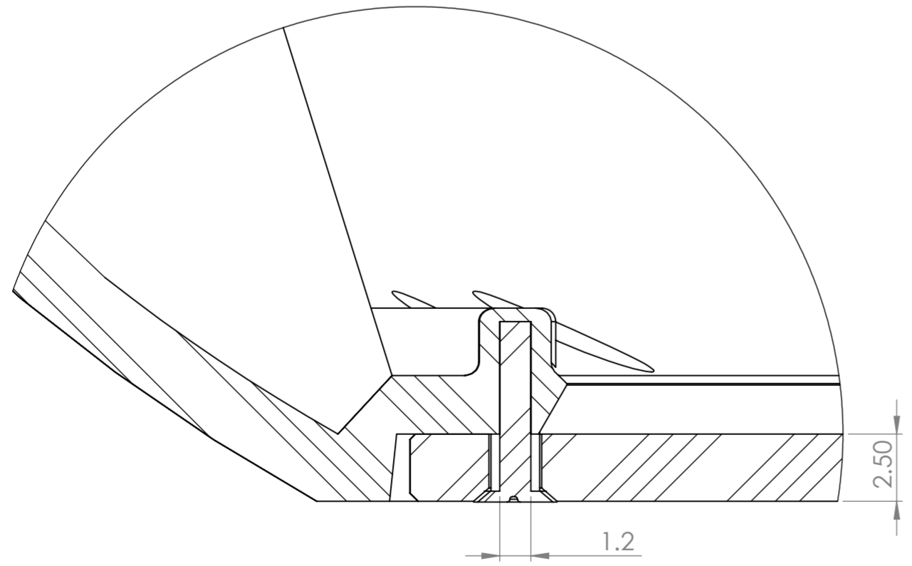
DETAIL C SCALE 5:1
