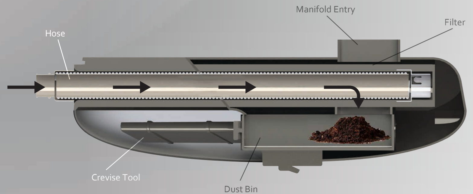
Cut section view of the mechanics of the vacuum system. The dirt path goes through the hose and down into the dust bin, while getting its suction from the manifold.
