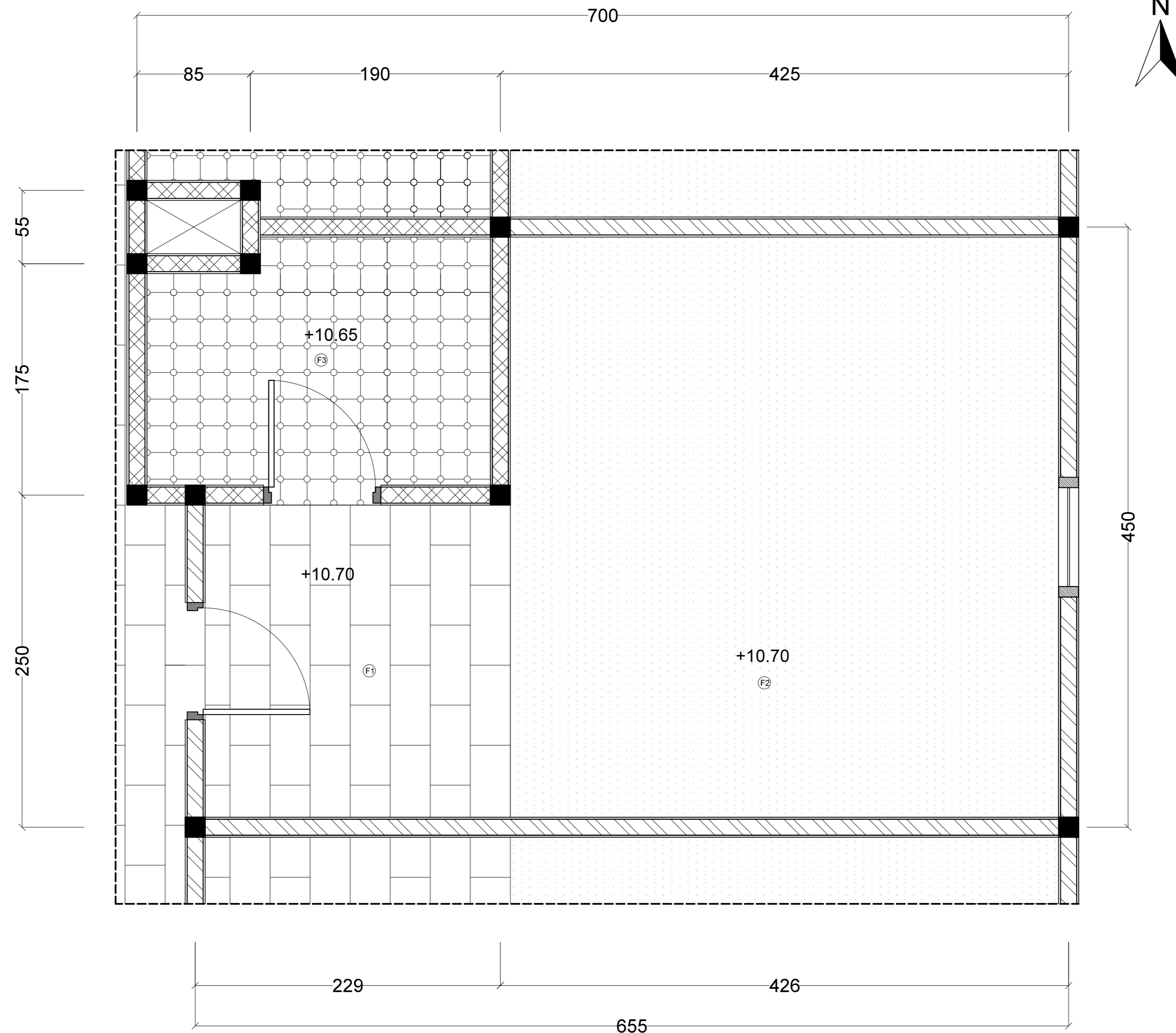
BUGINESE STANDARD BEDROOM FLOOR LAYOUT PLAN (2ND) SCALE 1 : 25
