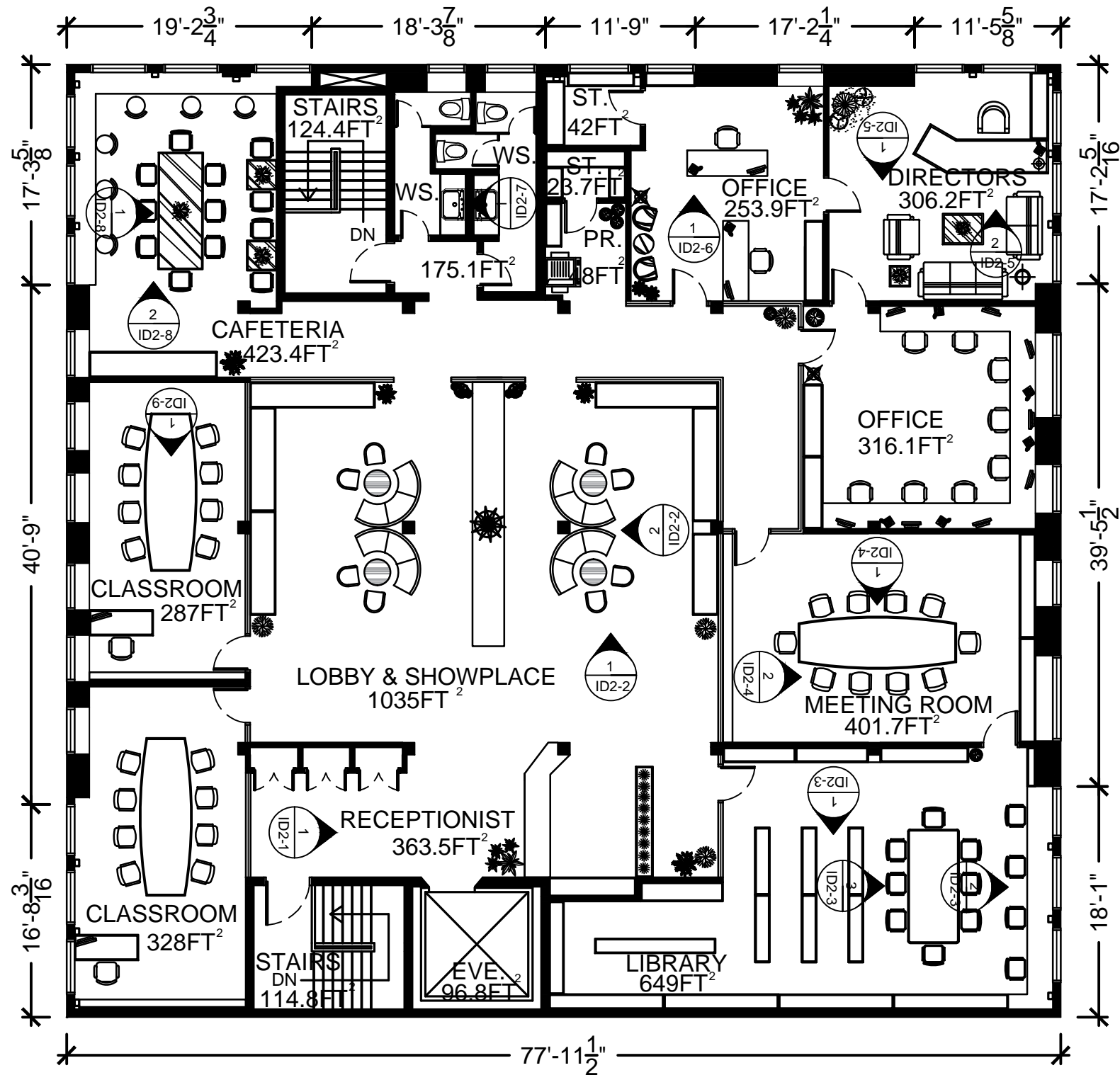
1 FLOOR PLAN 3/32"=1'-0"
