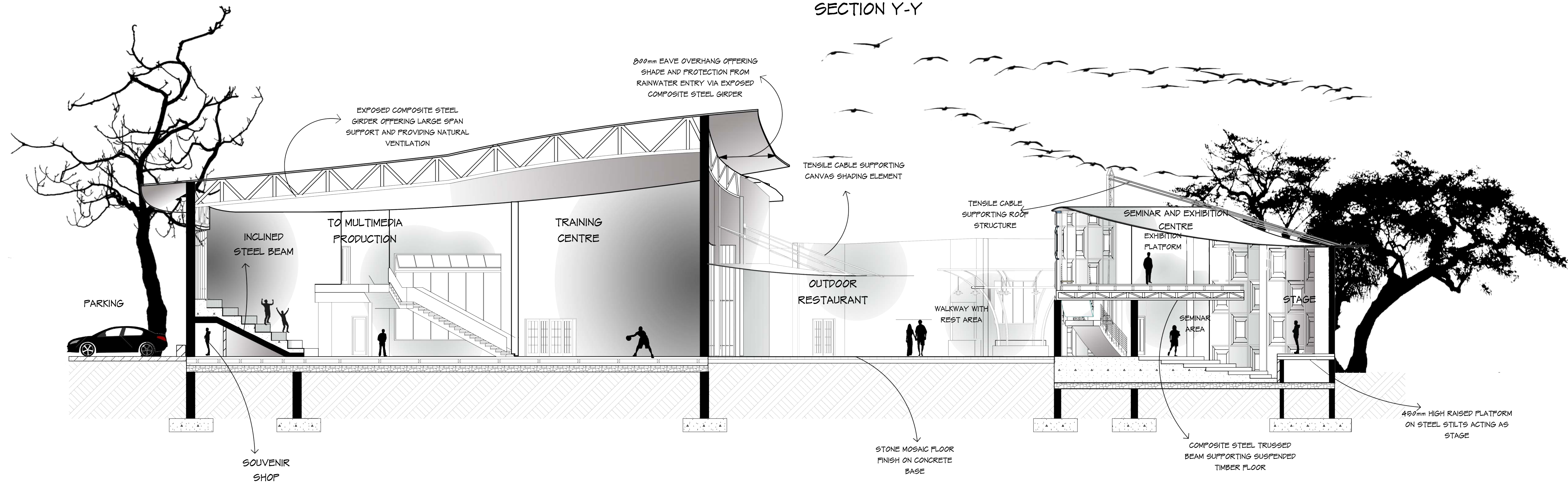
SECTION Y-Y
