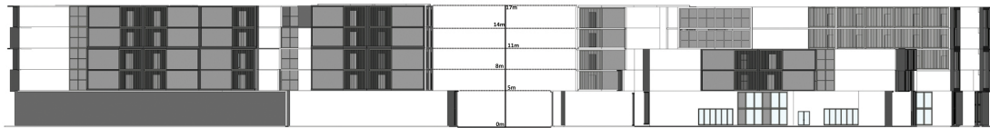
WEST ELEVATION
